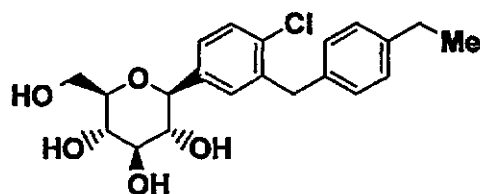
Compound 1 (a compound of formula I).
