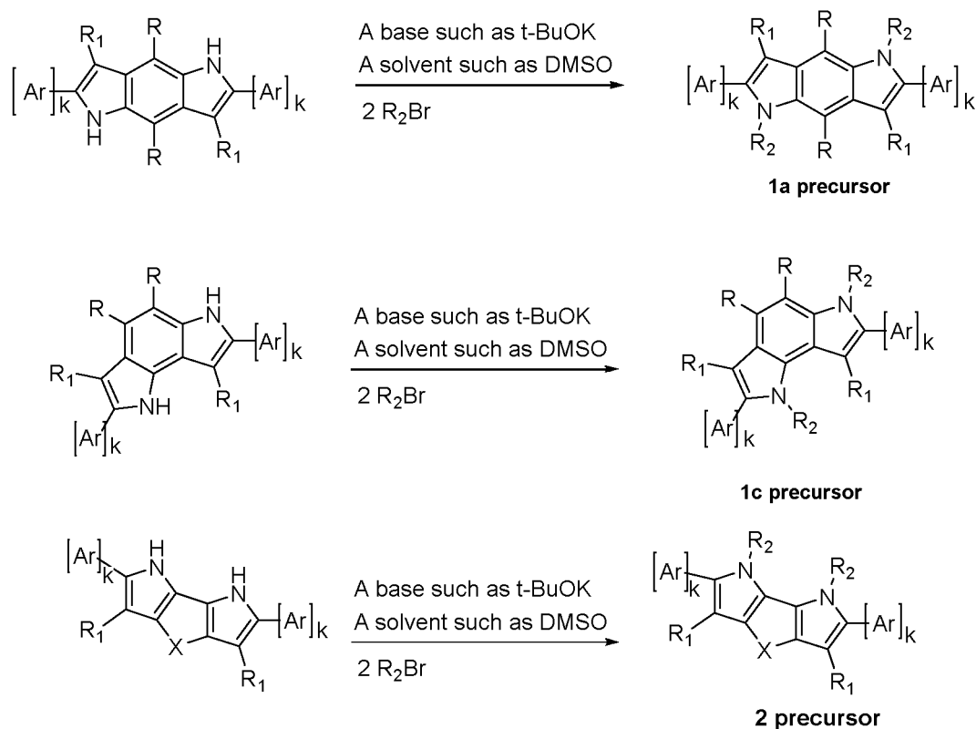
Scheme 4
