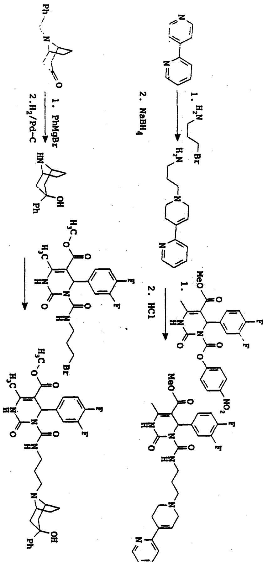
Scheme 20. Preparation of examples 44 and 52.
