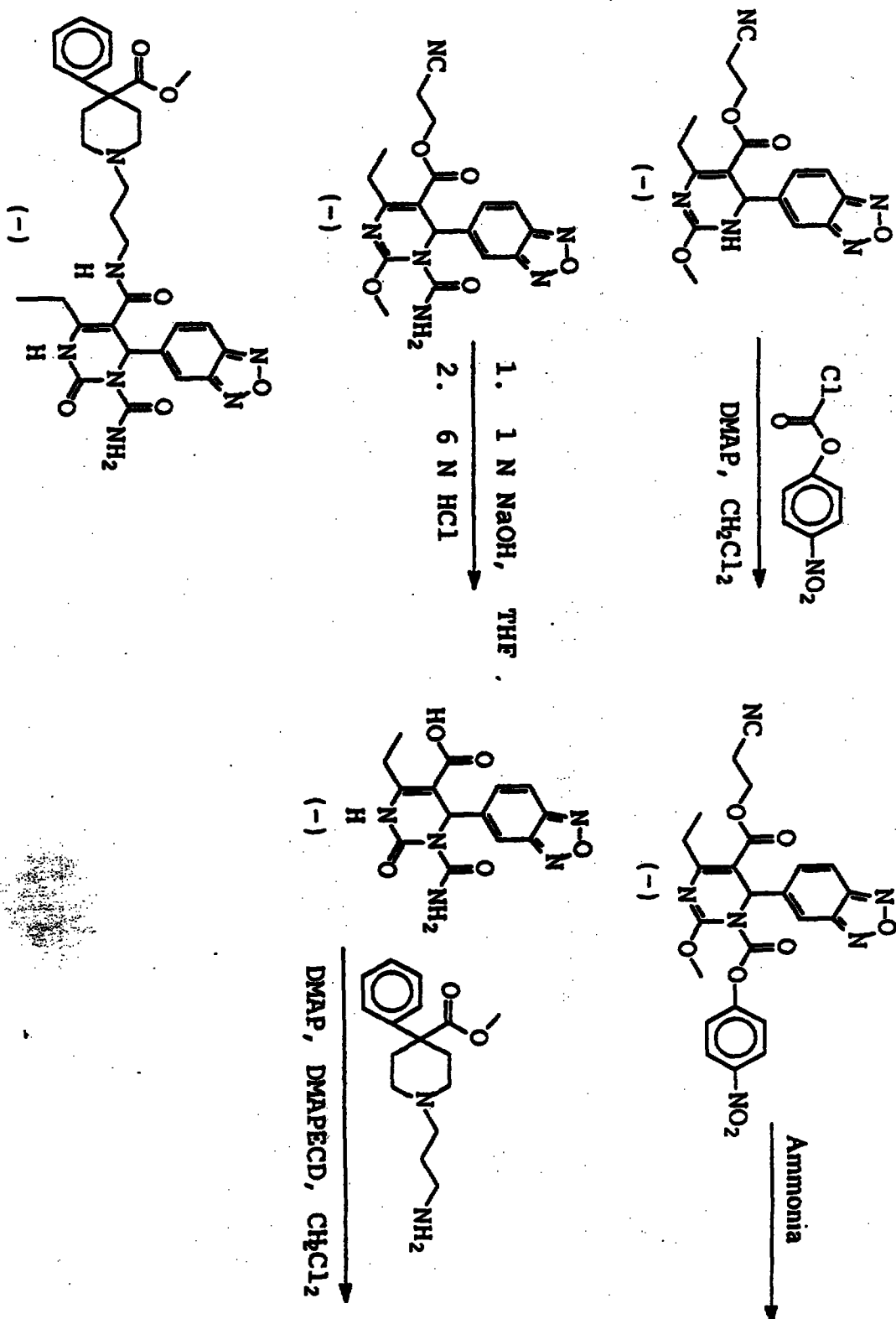
Scheme 13 (continued). Preparation of example 43 part-2
