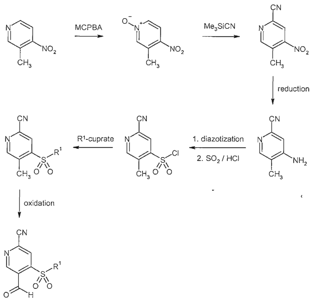
Scheme 8
