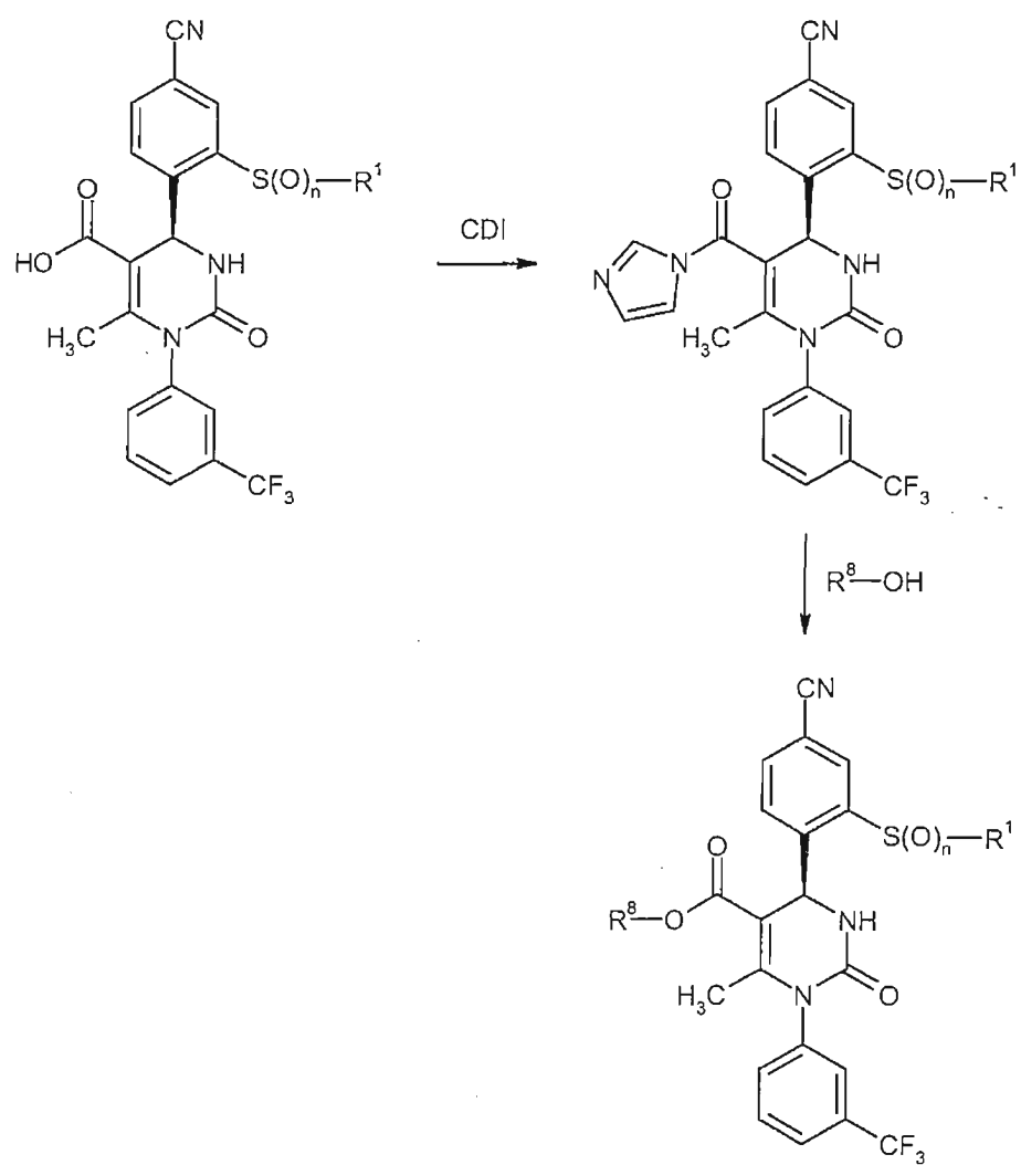
Scheme 3
