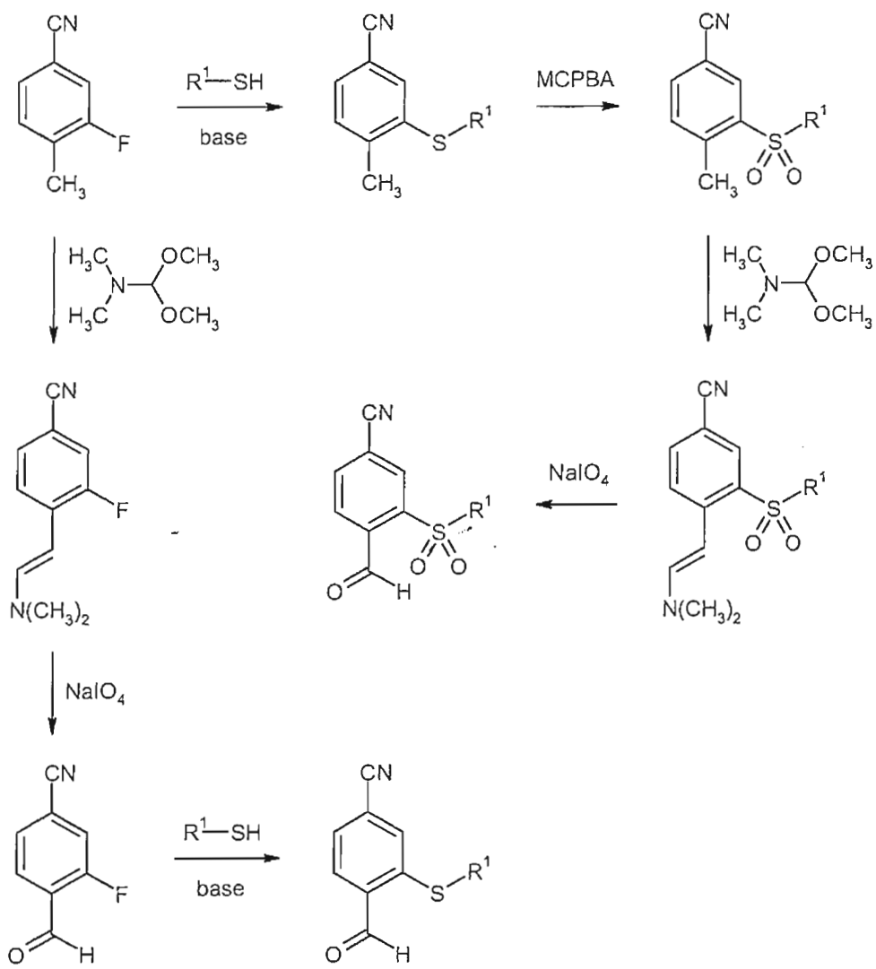
Scheme 6
