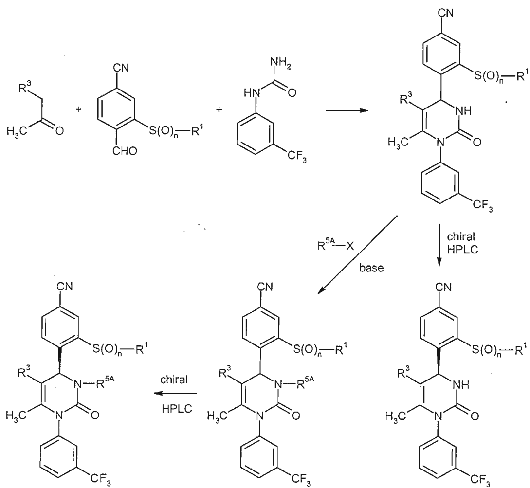
Scheme 1
