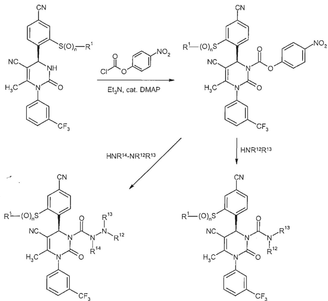
Scheme 4
