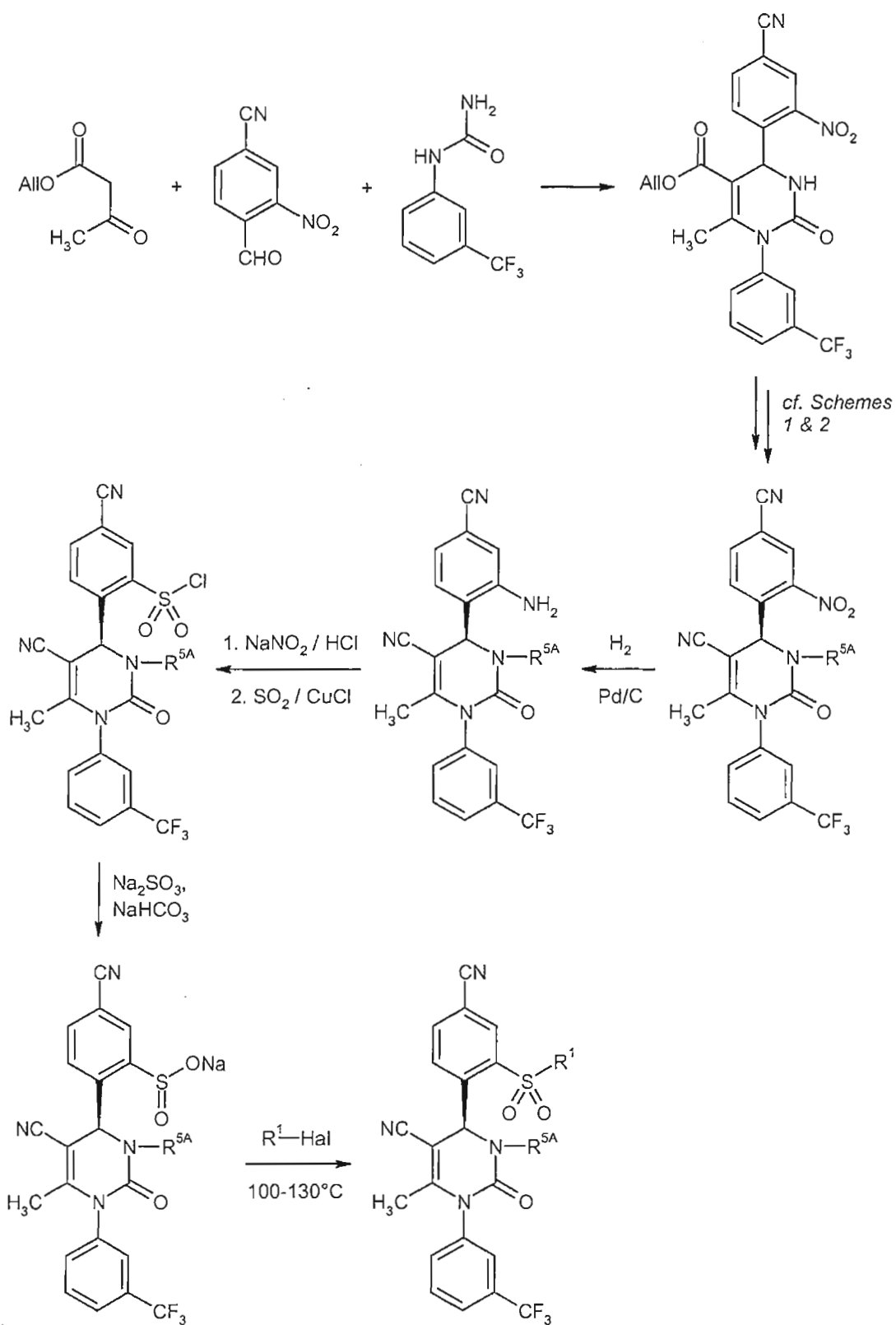
Scheme 10
