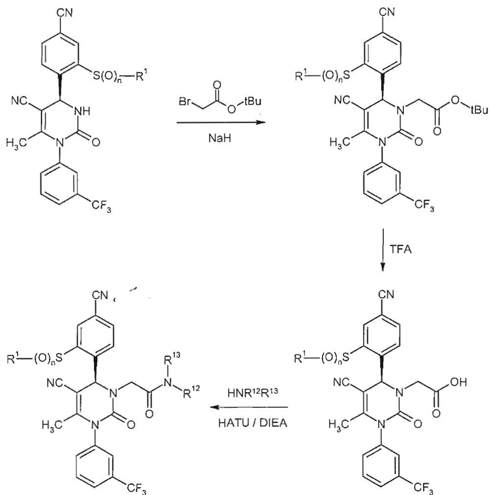
Scheme 5
