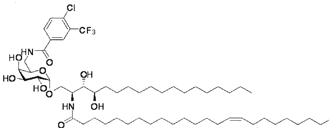
compound 6
