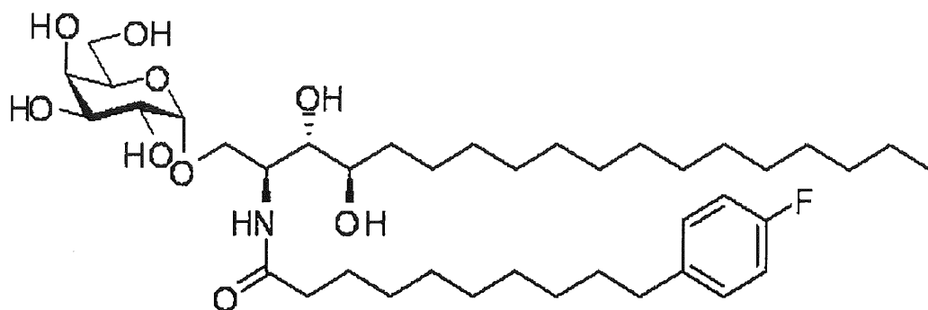
compound 7 (7DW8-5)
