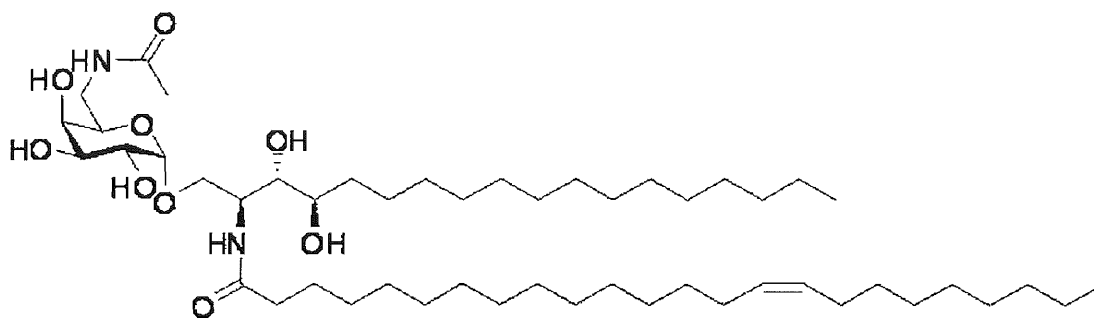
compound 5 (PBS-57)
