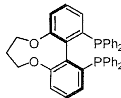
(S)-C3-TunePhos
