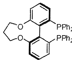
(R)-C3-TunePhos
