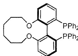
(S)-C6-TunePhos
