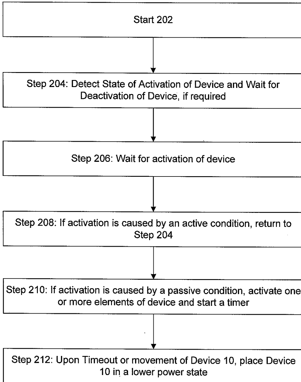
Algorithm 200
