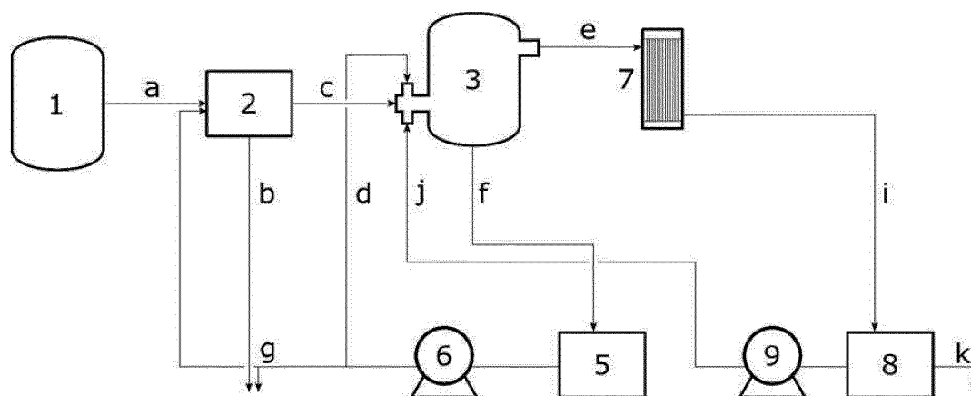
Figure 2: A screening assembly according to the second preferred embodiment of the present invention
