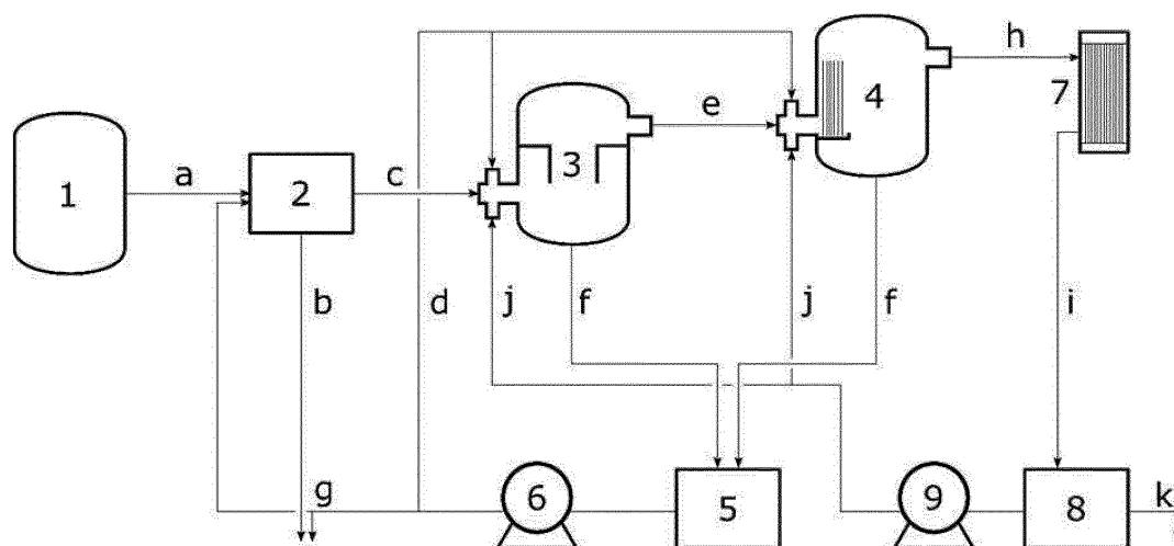
Figure 3: A screening assembly according to the third preferred embodiment of the present invention
