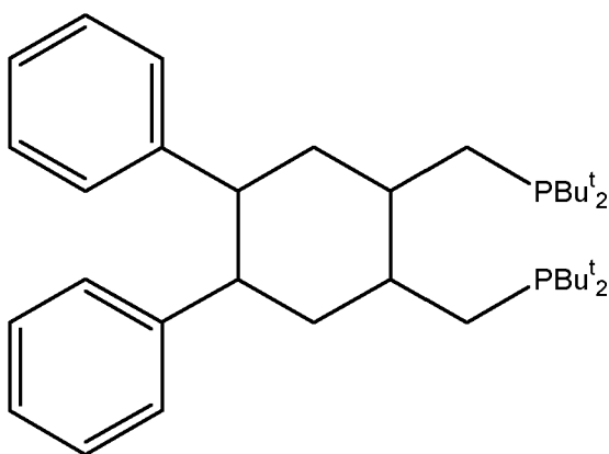
cis-1,2-bis(di-tert-butylphosphinomethyl)-4,5-diphenylcyclohexane
