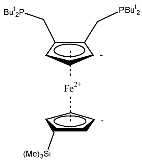
1,2-bis(di-tert-butylphosphinomethyl)-1'-trimethylsilyl ferrocene
