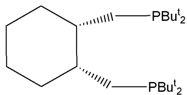
cis- 1, 2-bis (di-tert-butylphosphinomethyl) cyclohexane
