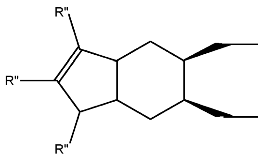
substituted 3a,
