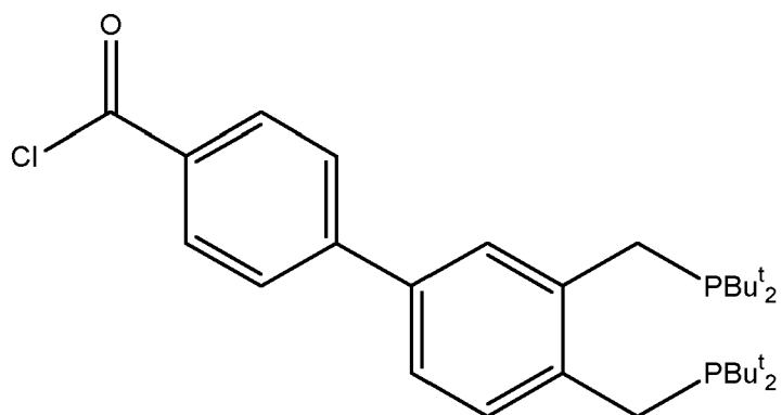
1,2-bis(di-tert-butyl (phosphinomethyl)-4-(4'-chlorocarbonyl-phenyl)benzene
