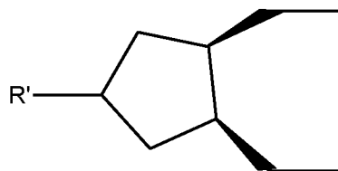
4 substituted
