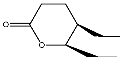
delta-valero lactone
