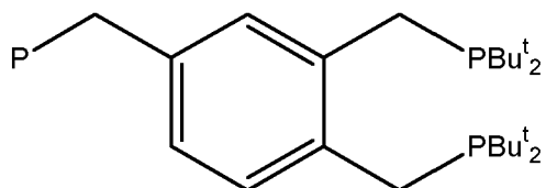
1,2-bis(di-tert-butyl (phosphinomethyl))-4-(phosphinomethyl)benzene
