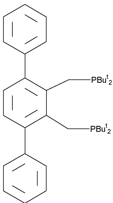
10 1, 2-bis (di-tert-butylphosphinomethyl)-3,6-diphenyl benzene
