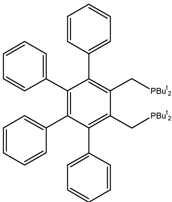
1,2-bis(di-tert-butyl(phosphinomethyl))-3,4,5,6-tetraphenyl benzene
