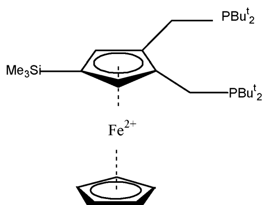
1,2-bis(di-tert-butylphospinomethyl)-4-trimethylsilyl ferrocene
