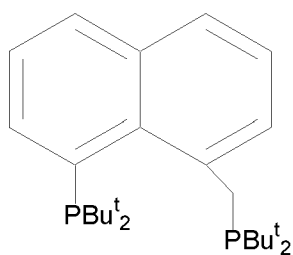
1-(di-tert-butylphosphino)-8-(di-tertbutylphosphinomethyl)-naphthalene
