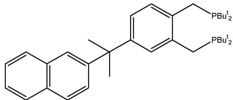
1,2-bis(di-tert-butyl (phosphinomethyl))-4-(phosphinomethyl)benzene
