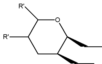
substituted tetrahydropyran
