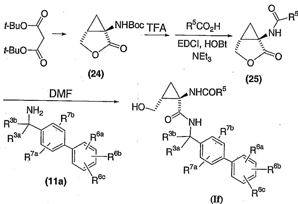
SCHEME 6
