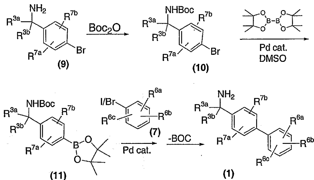
SCHEME 2b
