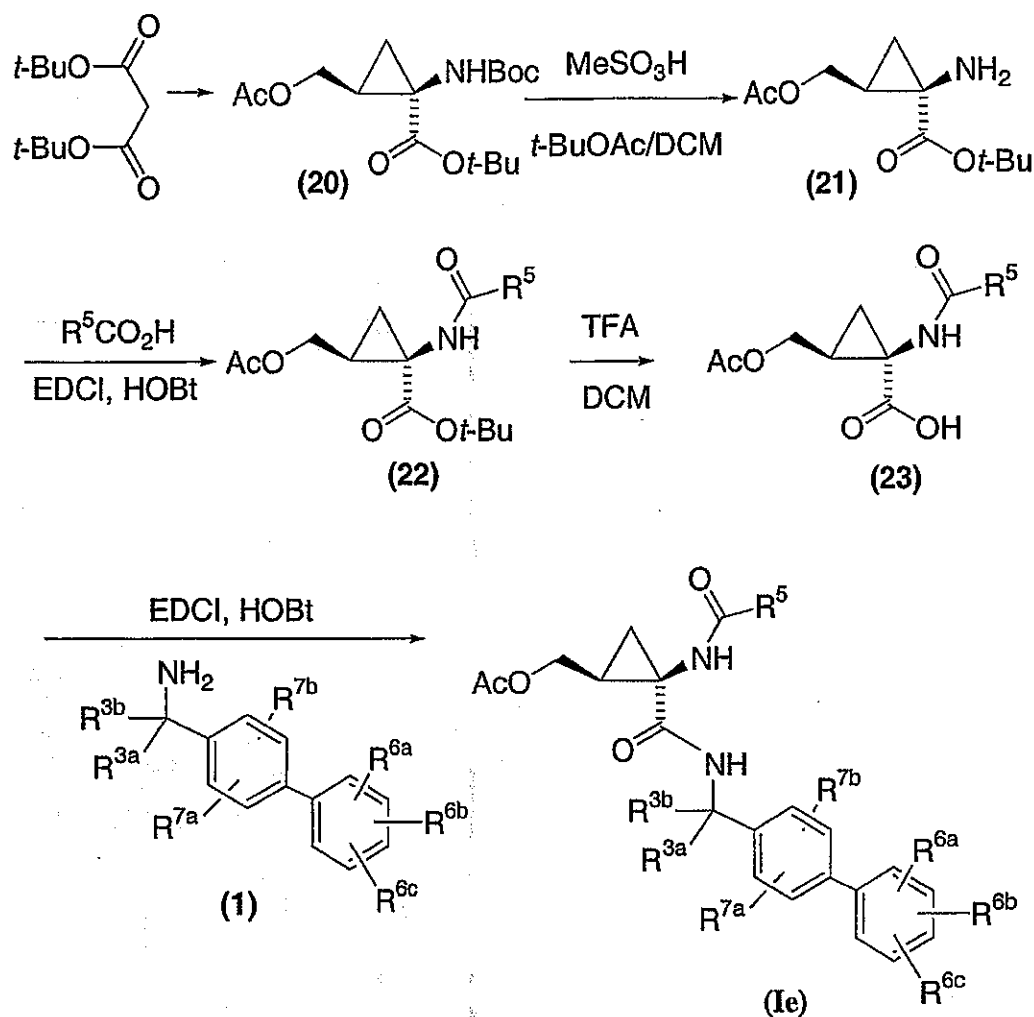
SCHEME 5
