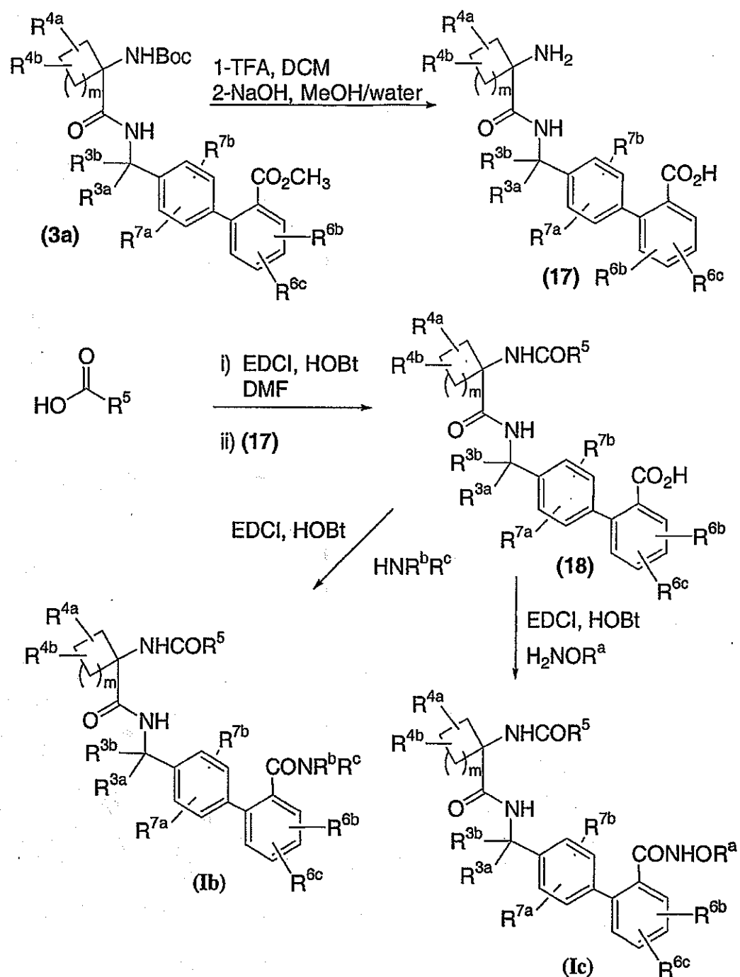
SCHEME 3
