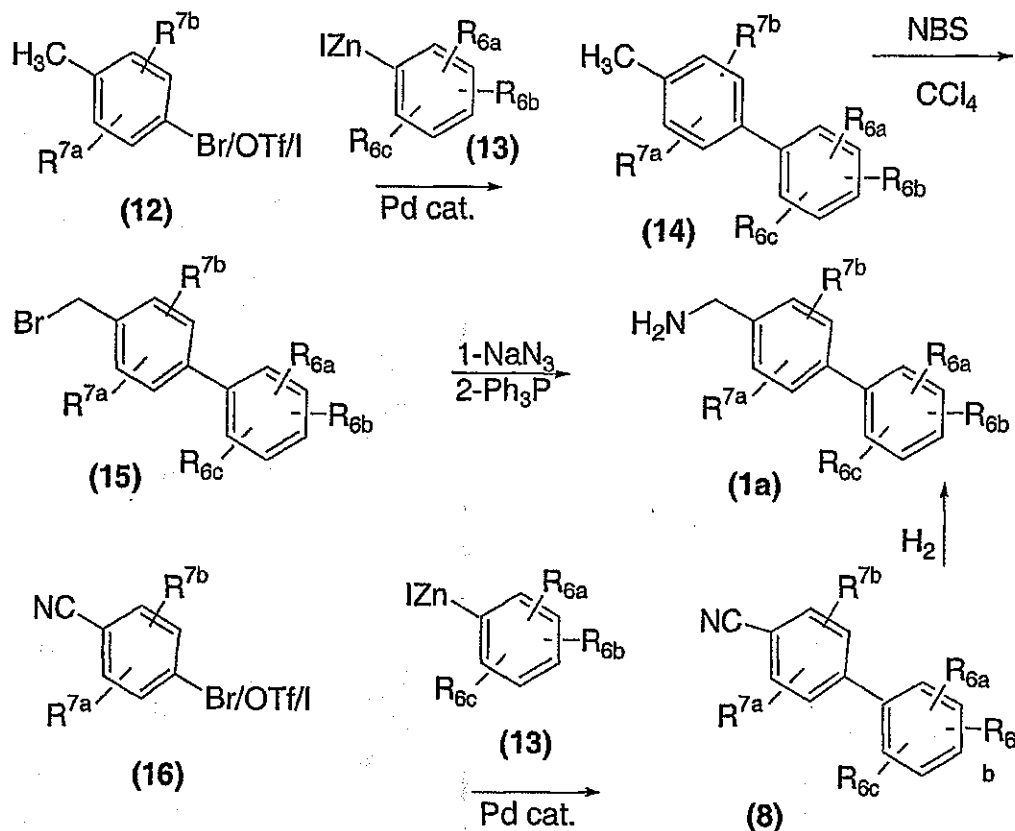
SCHEME 2c
