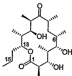
15-Methyl-6-deoxyerythronolide B
