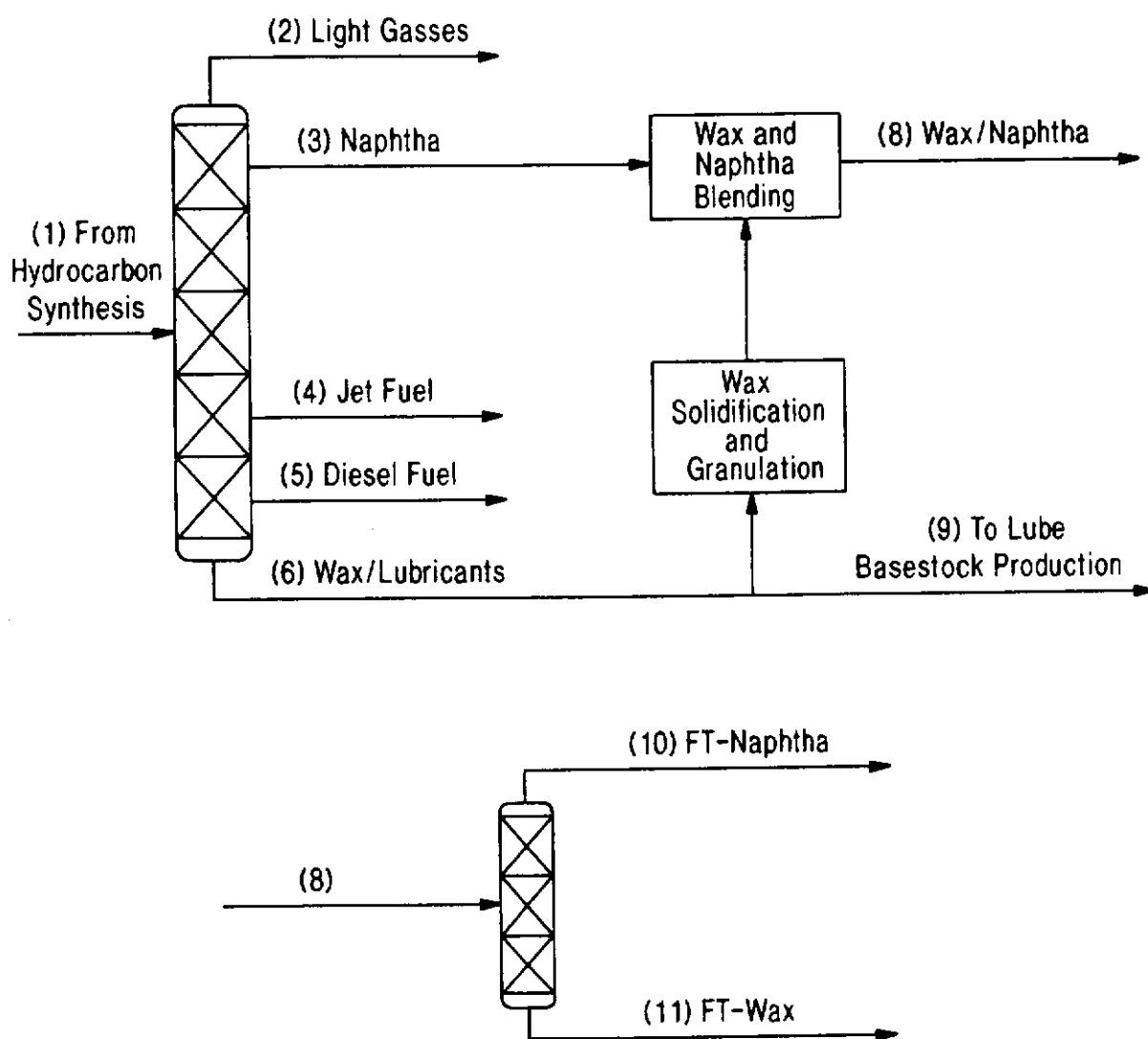
FT-Wax in FT-Naphtha Slurry Production Flow Scheme
