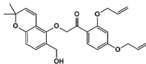
[Compound 4-64]
