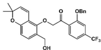
[Compound 4-59]
