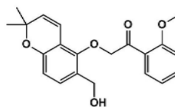
[Compound 4-60]
