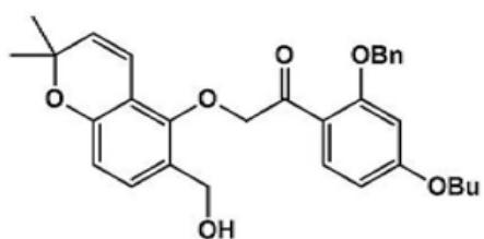
[Compound 4-7]
