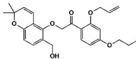
[Compound 4-42]
