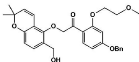
[Compound 4-16]
