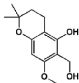
[Compound 2-6]
