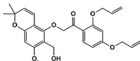
[Compound 4-62]
