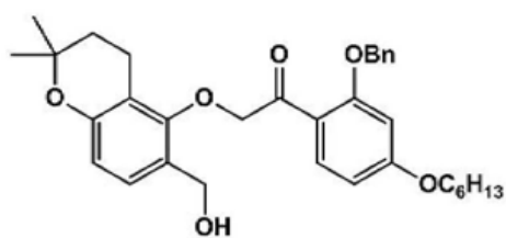
[Compound 4-75]
