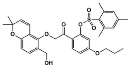
[Compound 4-43]
