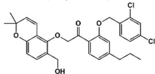
[Compound 4-24]
