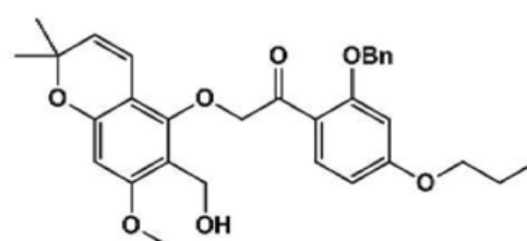
[Compound 4-48]
