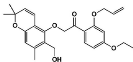
[Compound 4-59]
