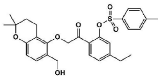
[Compound 4-103]
