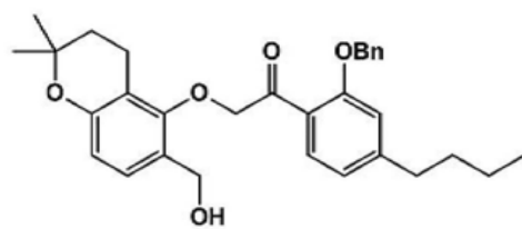
[Compound 4-93]
