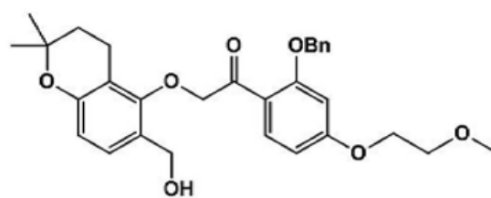
[Compound 4-76]
