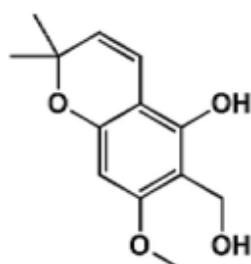
[Compound 2-5]
