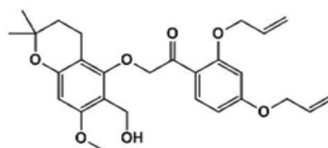
[Compound 4-128]
