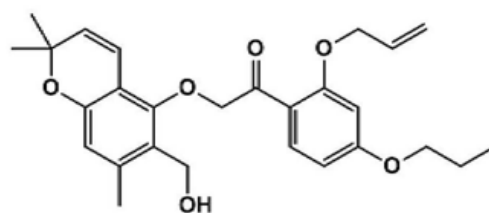
[Compound 4-60]
