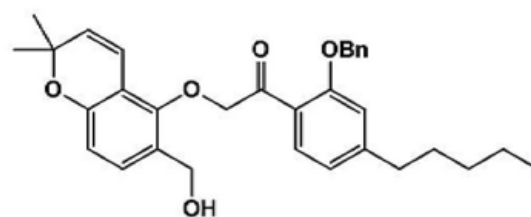
[Compound 4-28]
