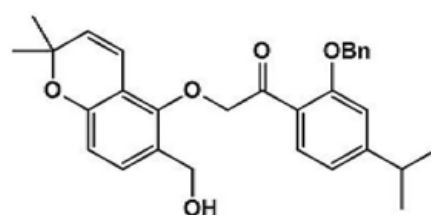
[Compound 4-26]
