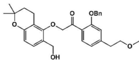
[Compound 4-95]
