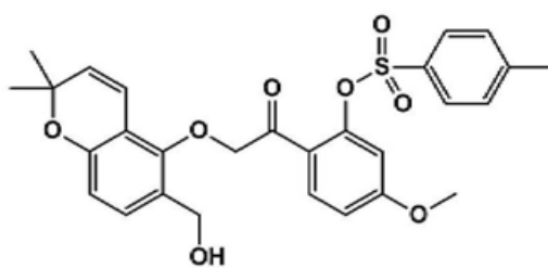
[Compound 4-55]
