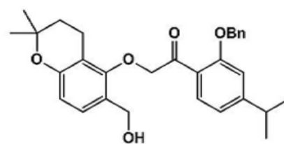
[Compound 4-92]
