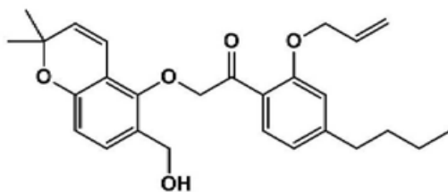
[Compound 4-53]
