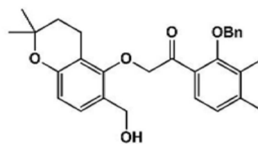
[Compound 4-96]
