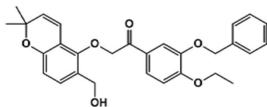
[Compound 4-61]
