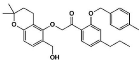
[Compound 4-89]
