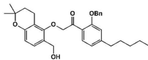
[Compound 4-94]
