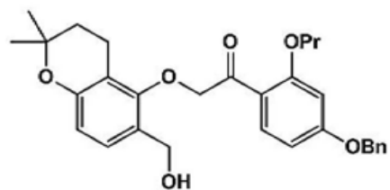
[Compound 4-80]
