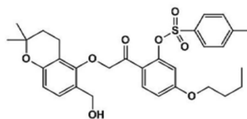
[Compound 4-112]
