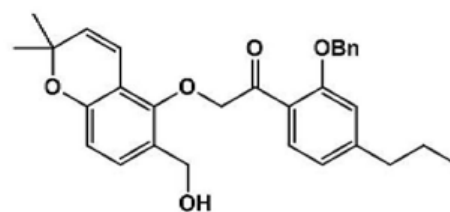
[Compound 4-20]
