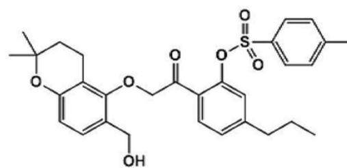
[Compound 4-104]
