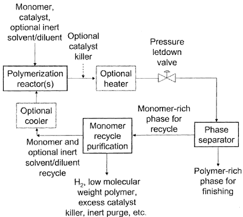
Figure 5. Process configuration for monomer recovery by phase separation
