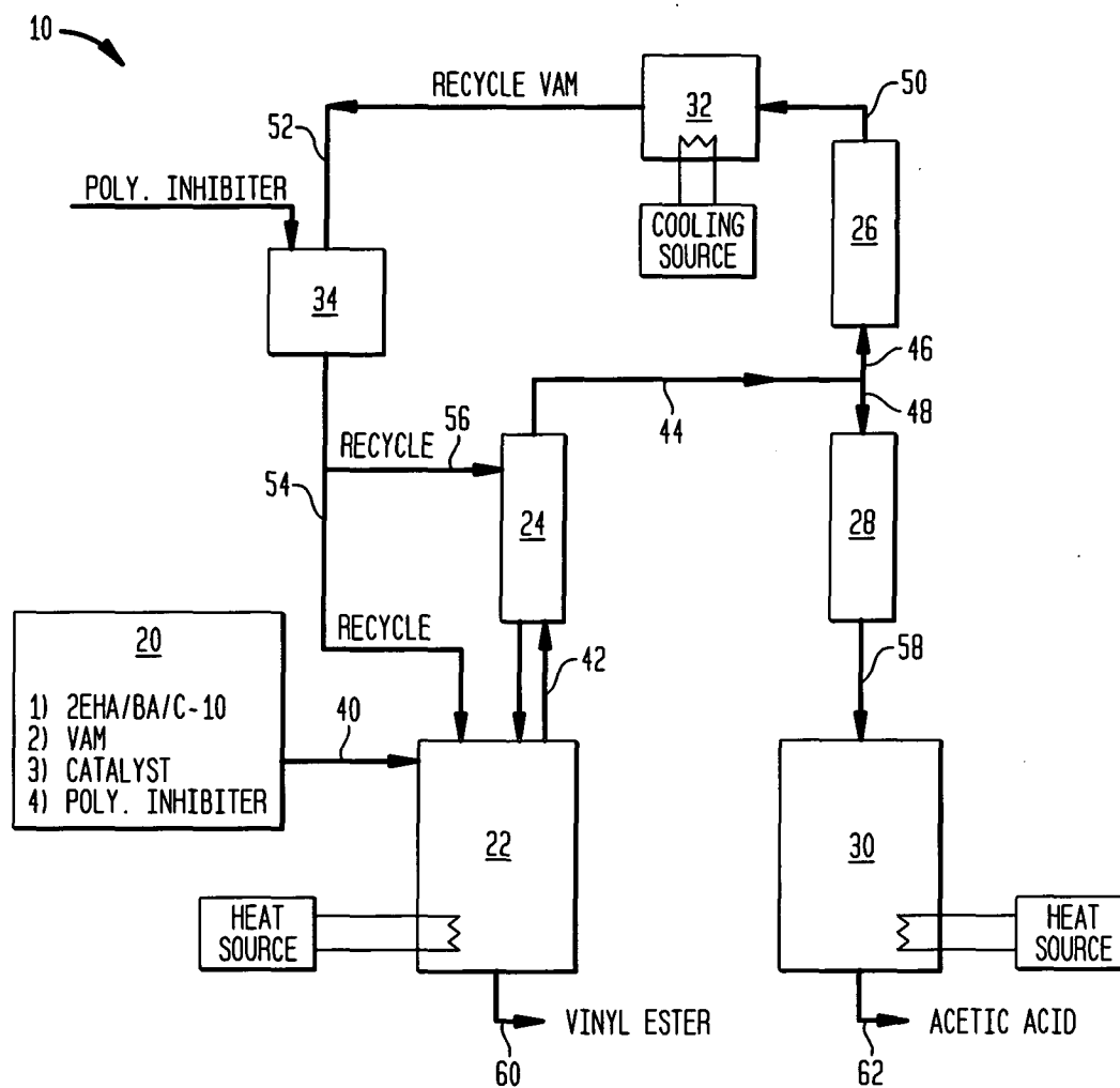
FIG. 1 SEMI CONTINUOUS TRANS-VINYLATION PROCESS
