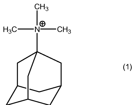
N,N,N-trimethyl-1-adamantammonium cation
