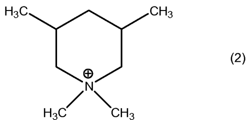
N,N-dimethyl-3,5-dimethylpiperidinium cation
