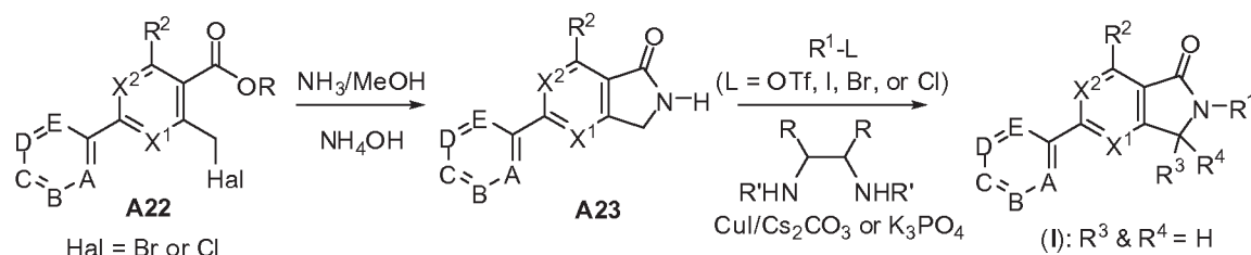
Scheme 1, Route F
