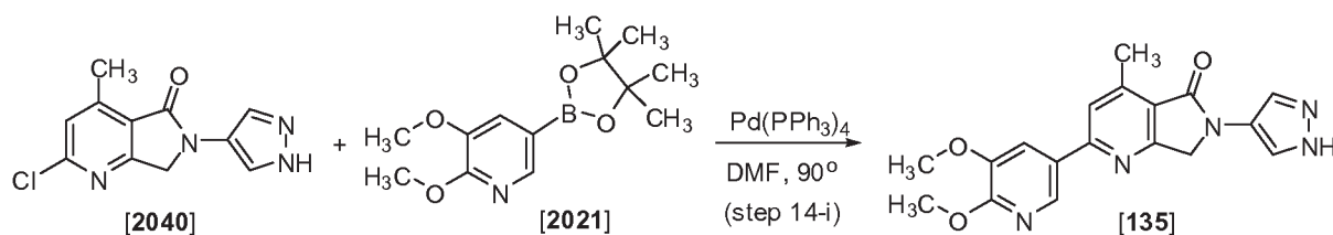
Scheme 12
