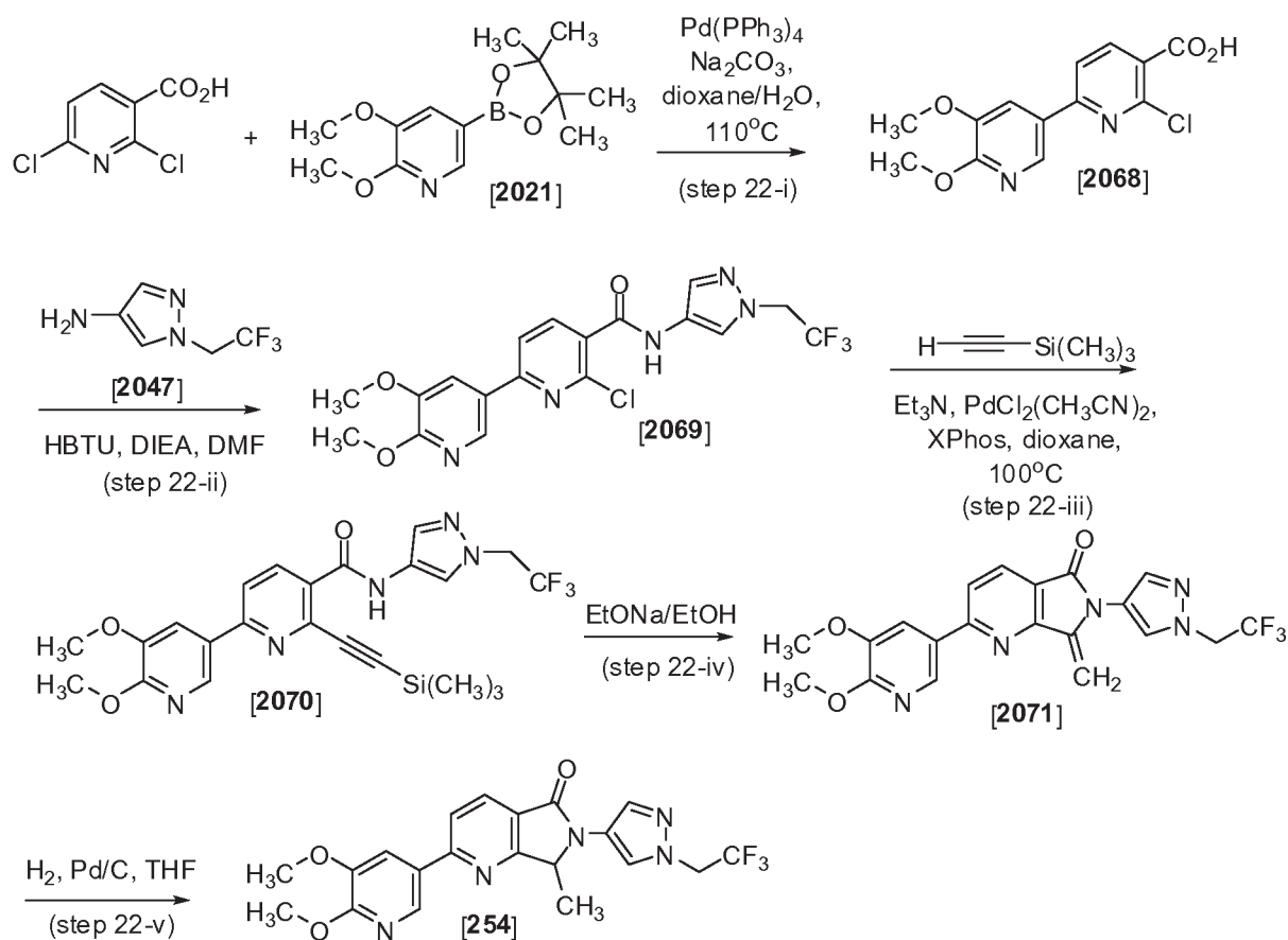
Scheme 22
