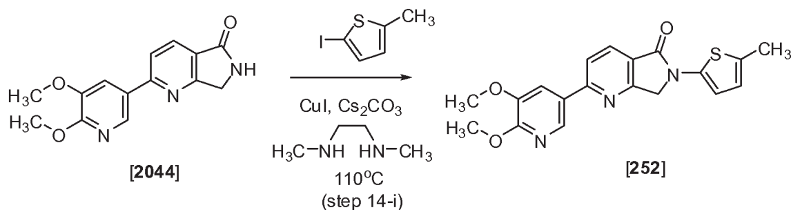
Scheme 14
