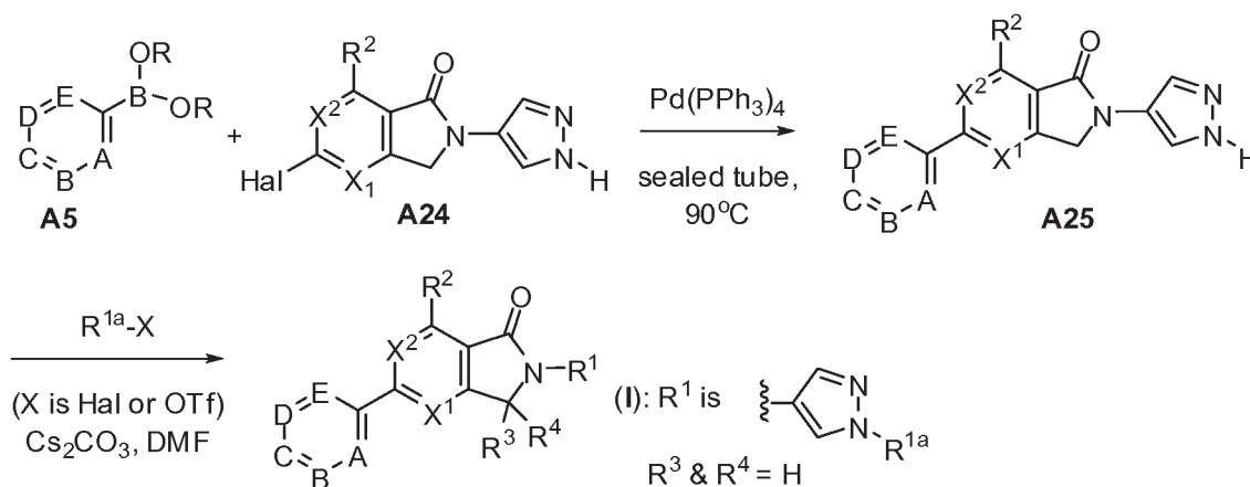
Scheme 1, Route G
