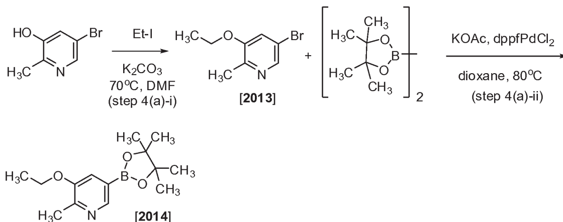
Scheme 4(a)
