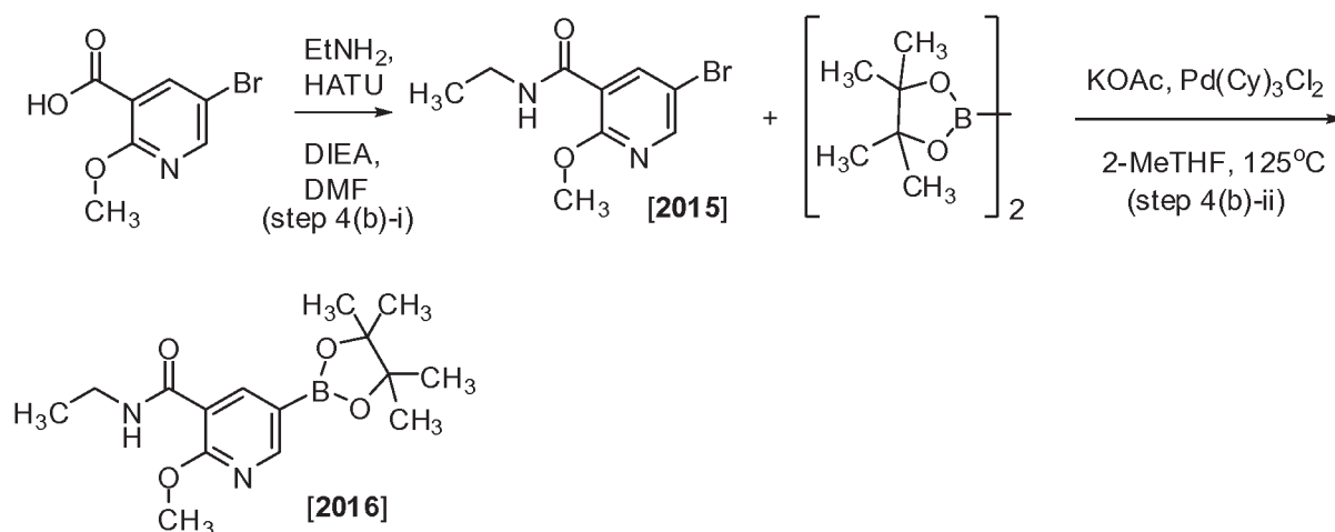
Scheme 4(b)
