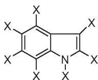
Structure b
