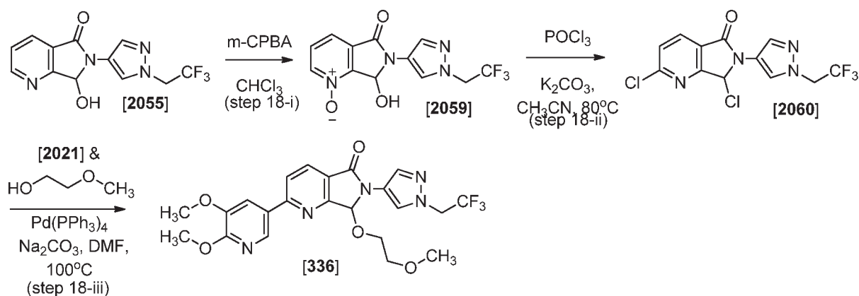
Scheme 18
