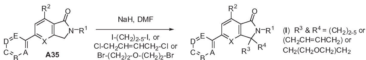
Scheme 1, Route K
