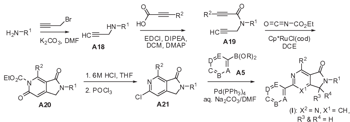
Scheme 1, Route E
