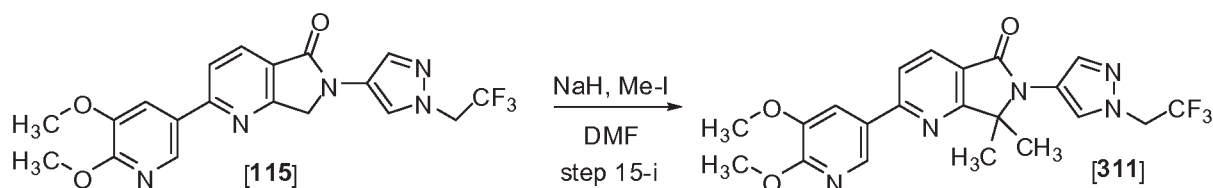
Scheme 15
