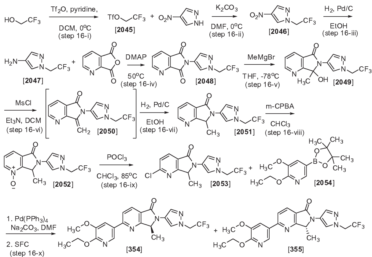
Scheme 16
