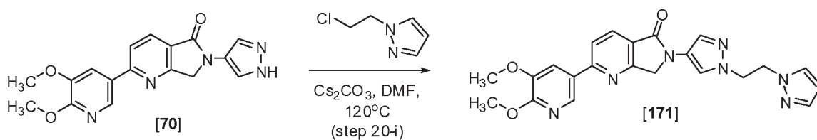
Scheme 20
