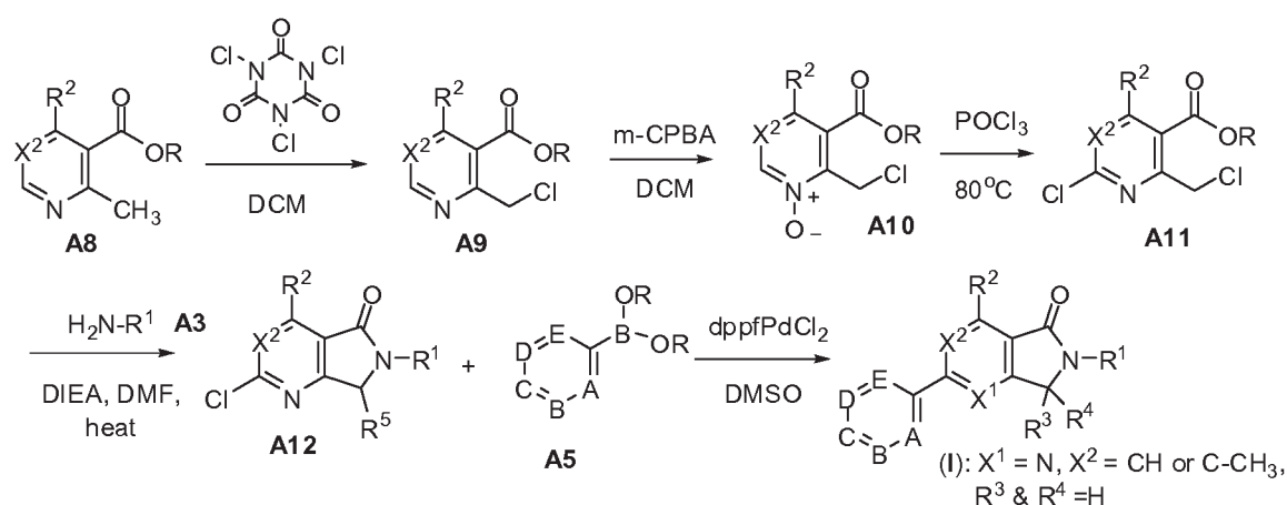
Scheme 1, Route C
