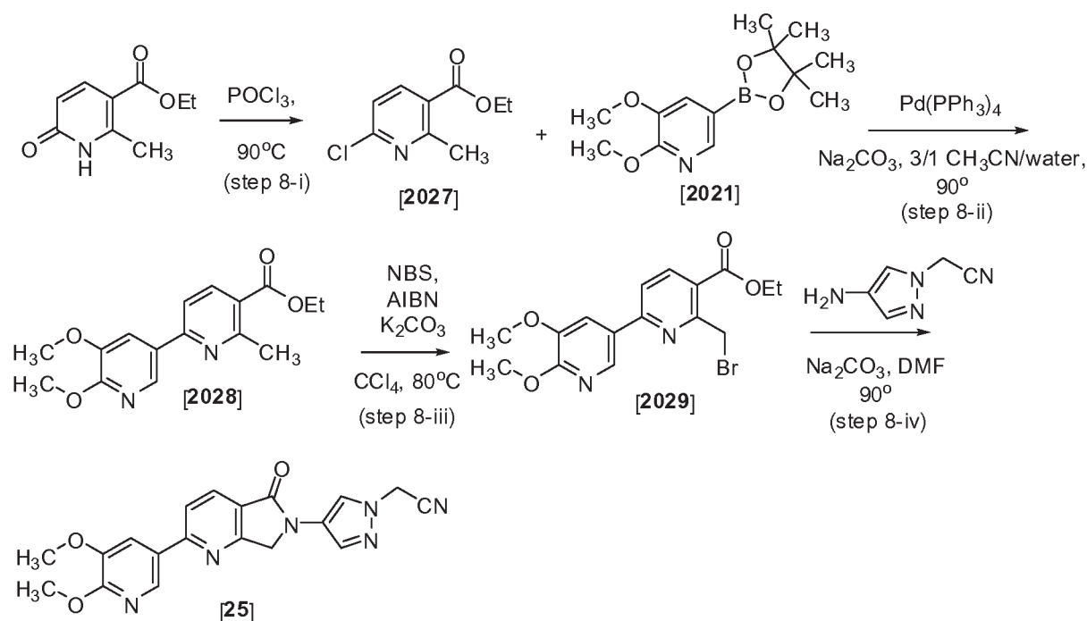
Scheme 8
