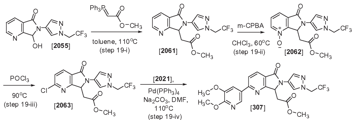
Scheme 19
