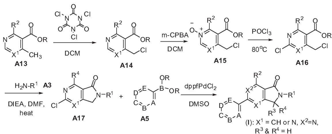
Scheme 1, Route D
