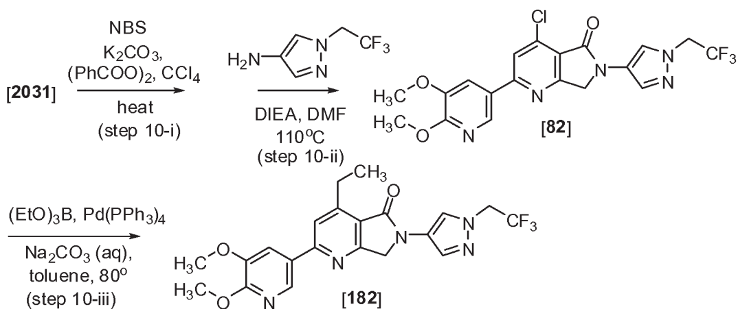
Scheme 10
