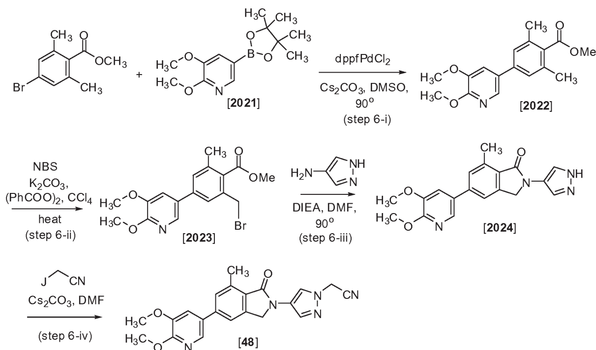
Scheme 6
