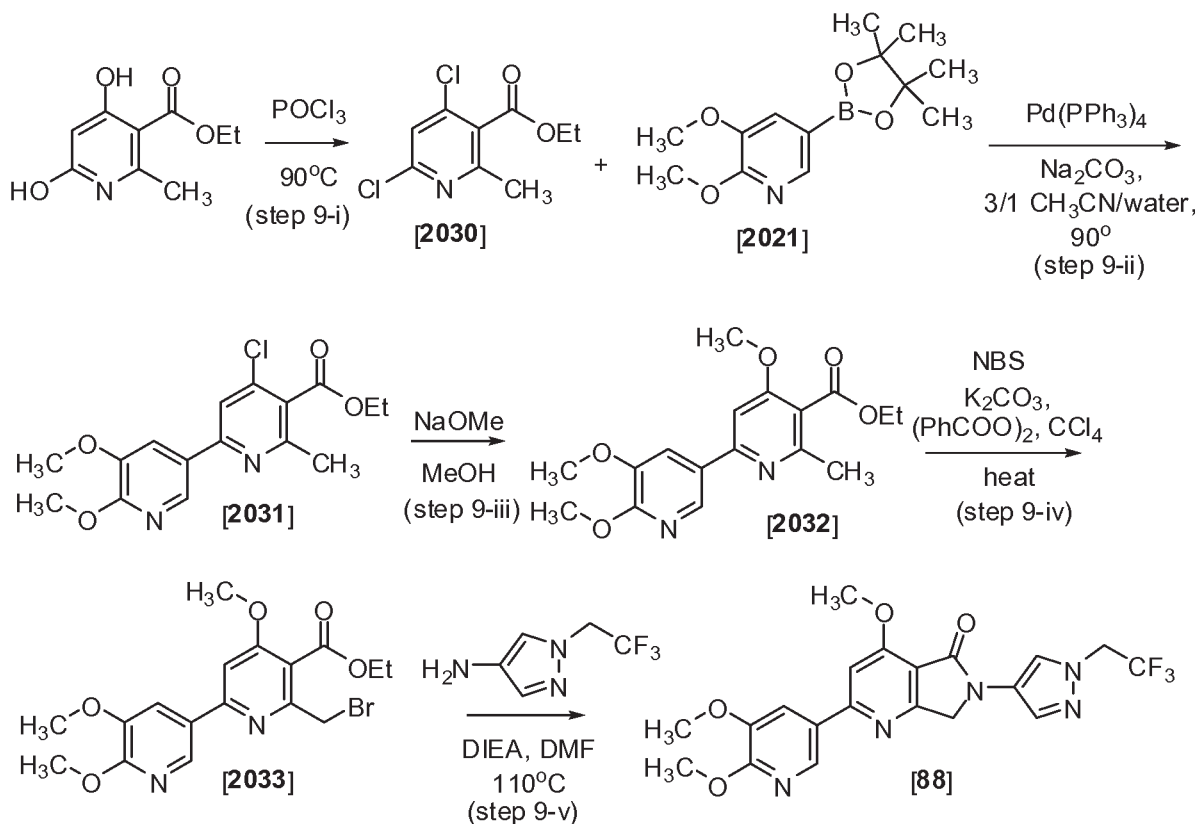
Scheme 9
