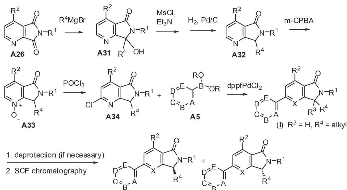
Scheme 1, Route I
