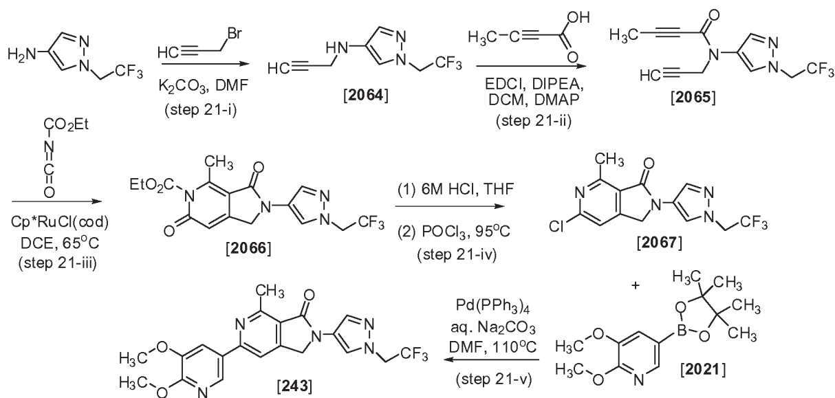
Scheme 21
