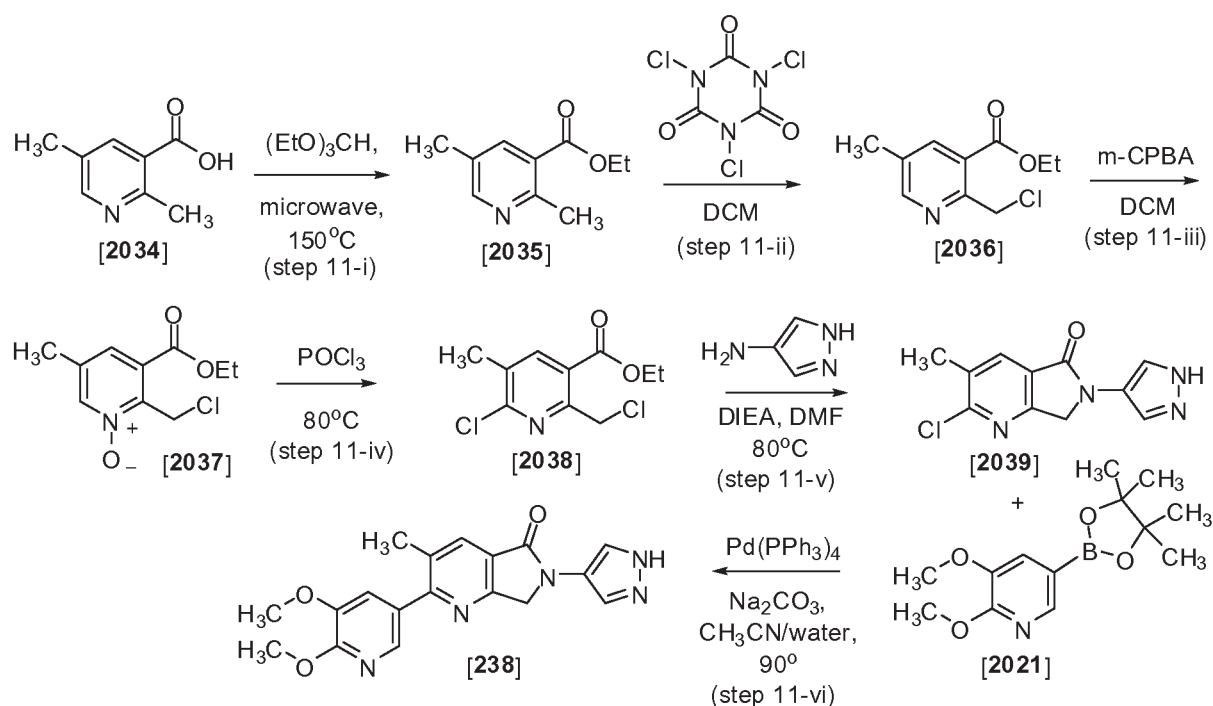
Scheme 11
