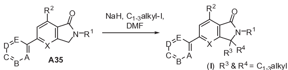
Scheme 1, Route J
