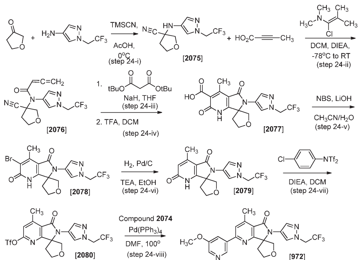
Scheme 24
