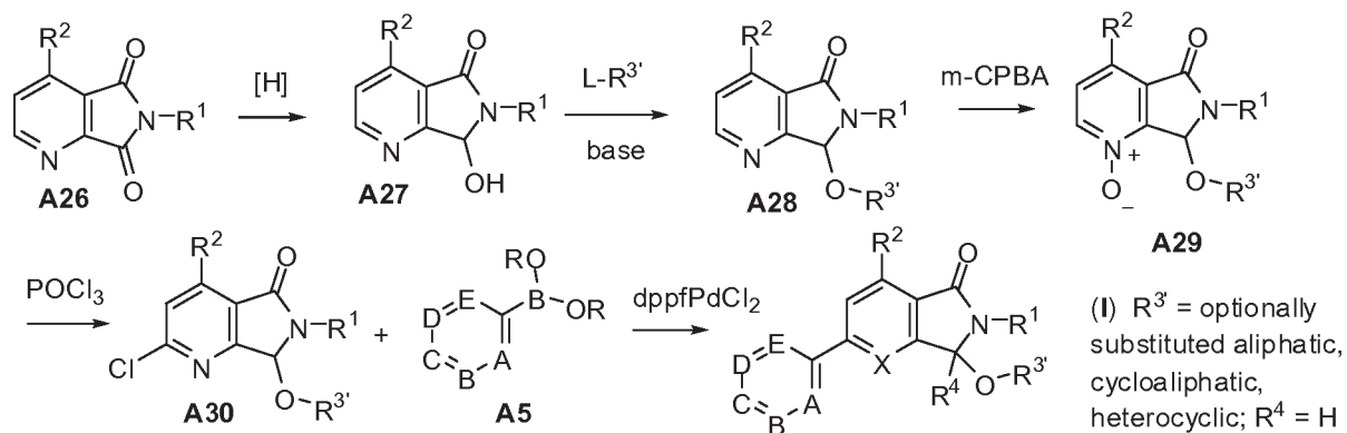
Scheme 1, Route H
