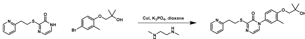
1-(4-(2-Hydroxy-2-methylpropoxy)-3-methylphenyl)-3-(2-(pyridin-2-yl)ethylthio)pyrazin-2(1H)-one
