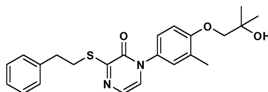
1-(4-(2-Hydroxy-2-methylpropoxy)-3-methylphenyl)-3-(phenethylthio)pyrazin-
