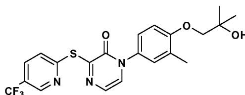
1-(4-(2-Hydroxy-2-methylpropoxy)-3-methylphenyl)-3-(5-(trifluoromethyl)pyridin-2-ylthio)pyrazin-2(1H)-one
