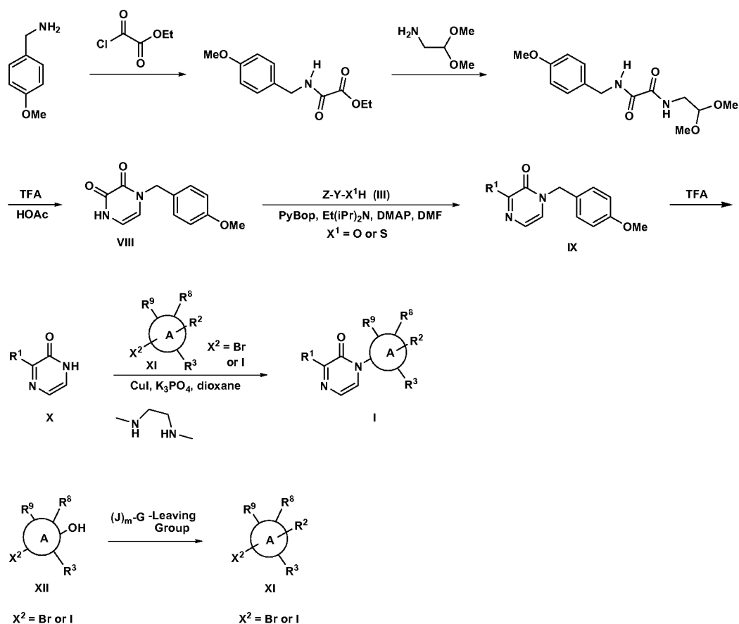
Scheme 2
