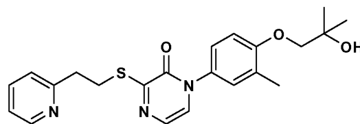
1-(4-(2-Hydroxy-2-methylpropoxy)-3-methylphenyl)-3-(2-(pyridin-2-yl)ethylthio)pyrazin-2(1H)-one
