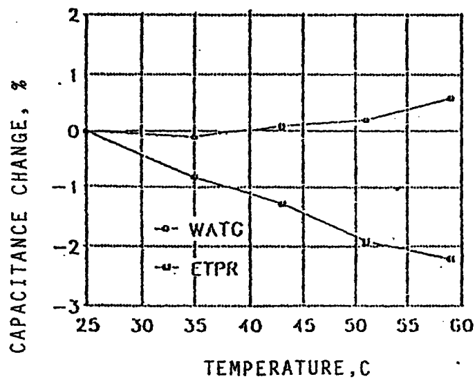
Figure 2 CABLE CAPACITANCE STABILITY AS A FUNCTION OF TEMPERATURE
