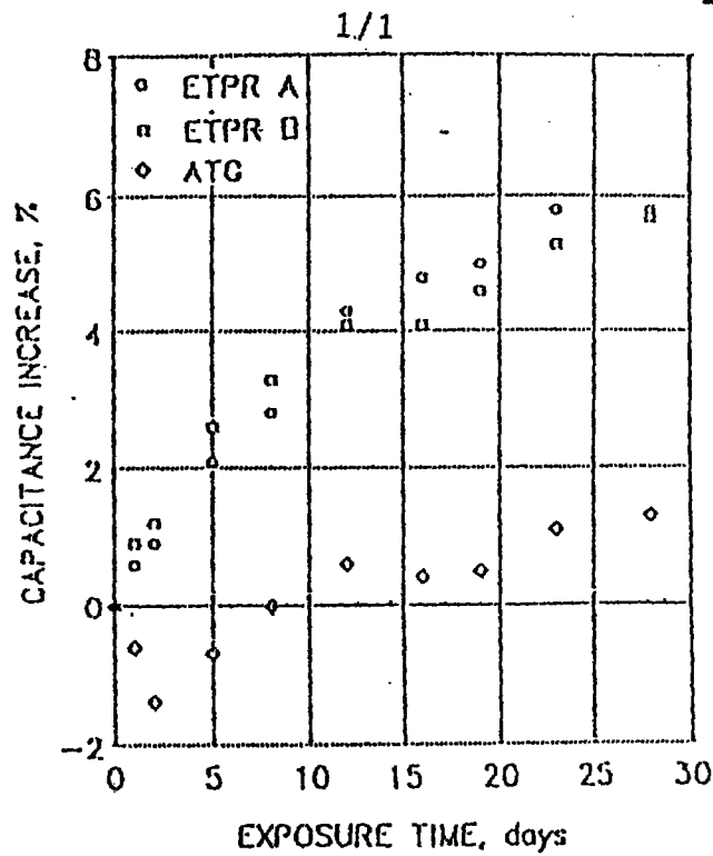
Figure 1 CAPACITANCE STABILITY OF 26 GAUGE FOAM-SKIN @ 60C
