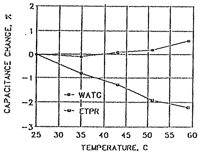
Figure 2 CABLE CAPACITANCE STABILITY AS A FUNCTION OF TEMPERATURE
