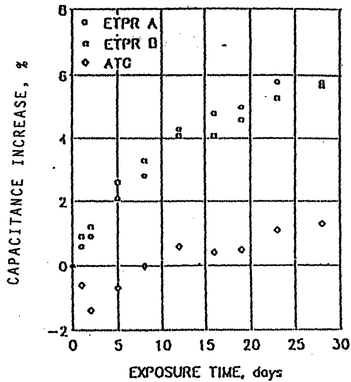
Figure 1 CAPACITANCE STABILITY OF 26 GAUGE FOAM-SKIN 60C
