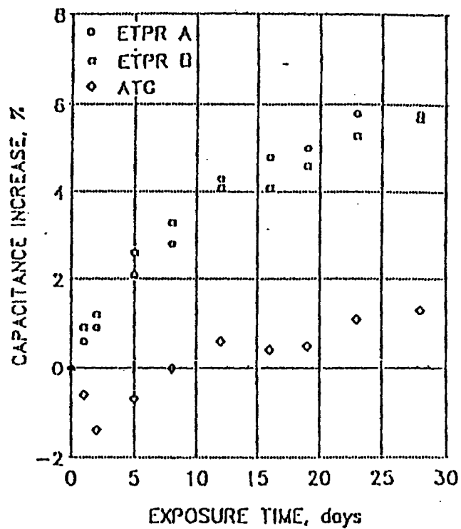
Figure 1 CAPACITANCE STABILITY OF 26 GAUGE FOAM-SKIN @ 60C
