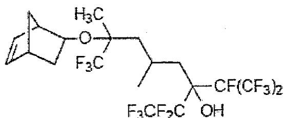
7-bicyclo[2.2.1]hept-5-en-2-yloxy-1,1,1,2,2,8,8,8-octafluoro-5,7-dimethyl-3-[1,2,2,2-tetrafluoro-1-(trifluoromethyl)ethyl]octan-3-ol
