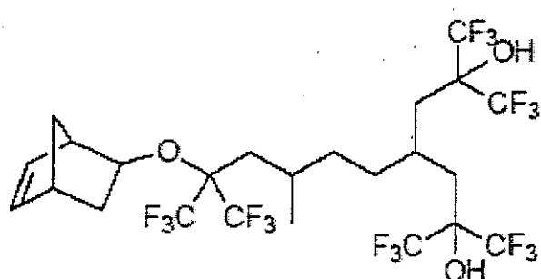
4-[5-bicyclo[2.2.1]hept-5-en-2-yloxy-6,6,6-trifluoro-3-methyl-5-(trifluoromethyl)hexyl]-2,6-bis(trifluoromethyl)-1,1,1,7,7,7-hexafluoroheptane-2,6-diol
