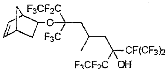
7-bicyclo[2.2.1]hept-5-en-2-yloxy-1,1,1,2,2,8,8,9,9,9-decafluoro-5-methyl-3-[1,2,2,2-tetrafluoro-1-(trifluoromethyl)ethyl]-7-(trifluoromethyl)nonan-3-ol
