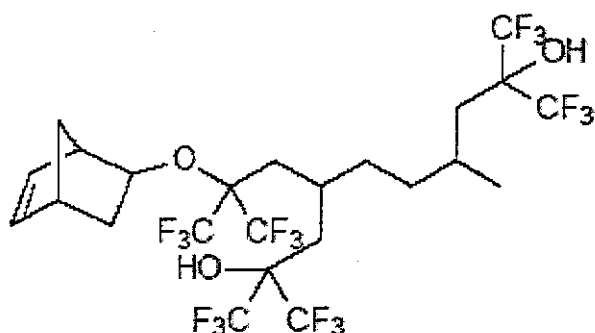
4-[2-bicyclo[2.2.1]hept-5-en-2-yloxy-3,3,3-trifluoro-2-(trifluoromethyl)propyl]-2,9-bis(trifluoromethyl)-1,1,1,10,10,10-hexafluoro-7-methyldecane-2,9-diol
