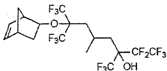
7-bicyclo[2.2.1]hept-5-en-2-yloxy-3,7-bis(trifluoromethyl)-1,1,1,2,2,8,8,8-octafluoro-5-methyloctan-3-ol
