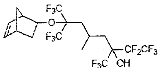
7-bicyclo[2.2.1]hept-5-en-2-yloxy-3,7-bis(trifluoromethyl)-1,1,1,2,2,8,8,8-octafluoro-5-methyloctan-3-ol
