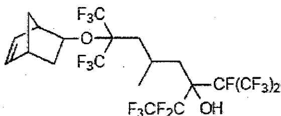
7-bicyclo[2.2.1]hept-5-en-2-yloxy-1,1,1,2,2,8,8,8-octafluoro-5-methyl-3-[1,2,2,2-tetrafluoro-1-(trifluoromethyl)ethyl]-7-(trifluoromethyl)octan-3-ol
