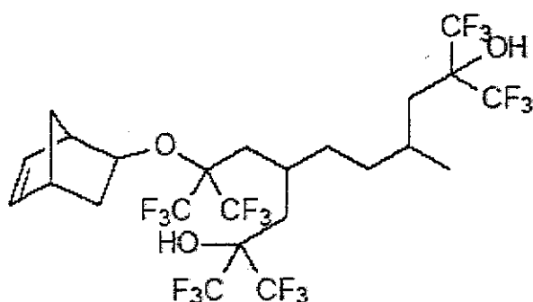
4-[2-bicyclo[2.2.1]hept-5-en-2-yloxy-3,3,3-trifluoro-2-(trifluoromethyl)propyl]-2,9-bis(trifluoromethyl)-1,1,1,10,10,10-hexafluoro-7-methyldecane-2,9-diol
