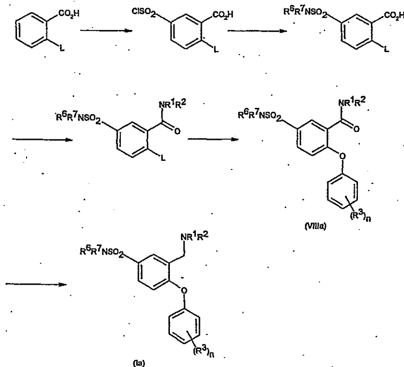
SCHEME 6
