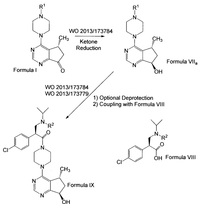
Scheme 5
