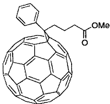
C 60 PCBM
