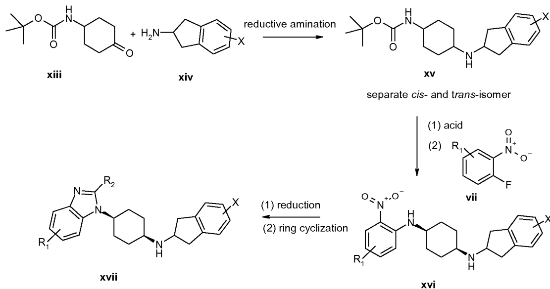
Scheme 4: Alternative method of coupling indane with benzoimidazole
