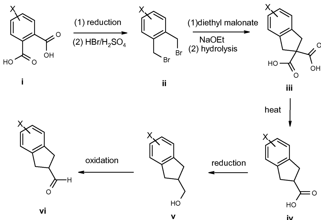
Scheme 1: General method of preparing substituted indan-2-carbaldehyde
