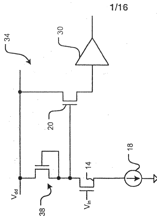
FIG. 2 Prior Art
