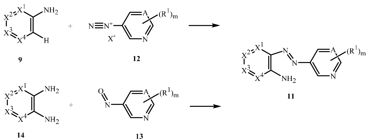
Scheme 7
