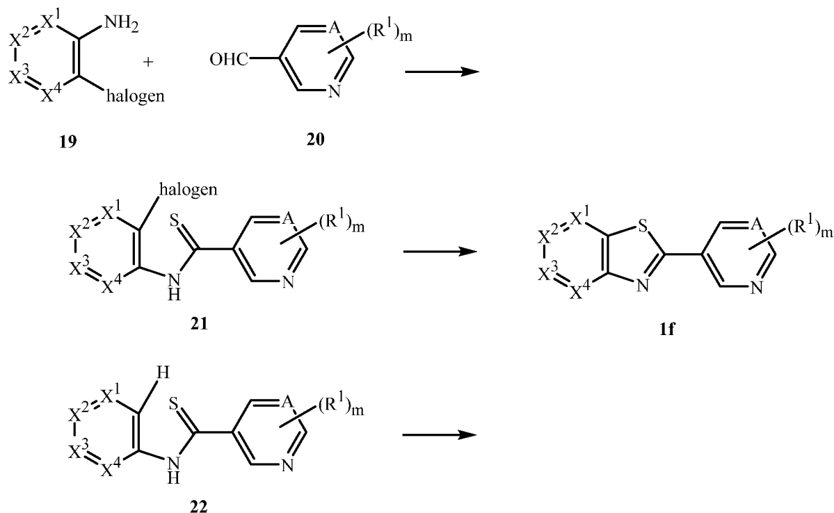
Scheme 12
