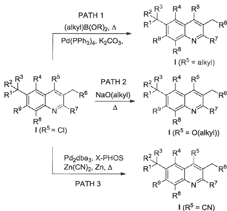
Scheme 8
