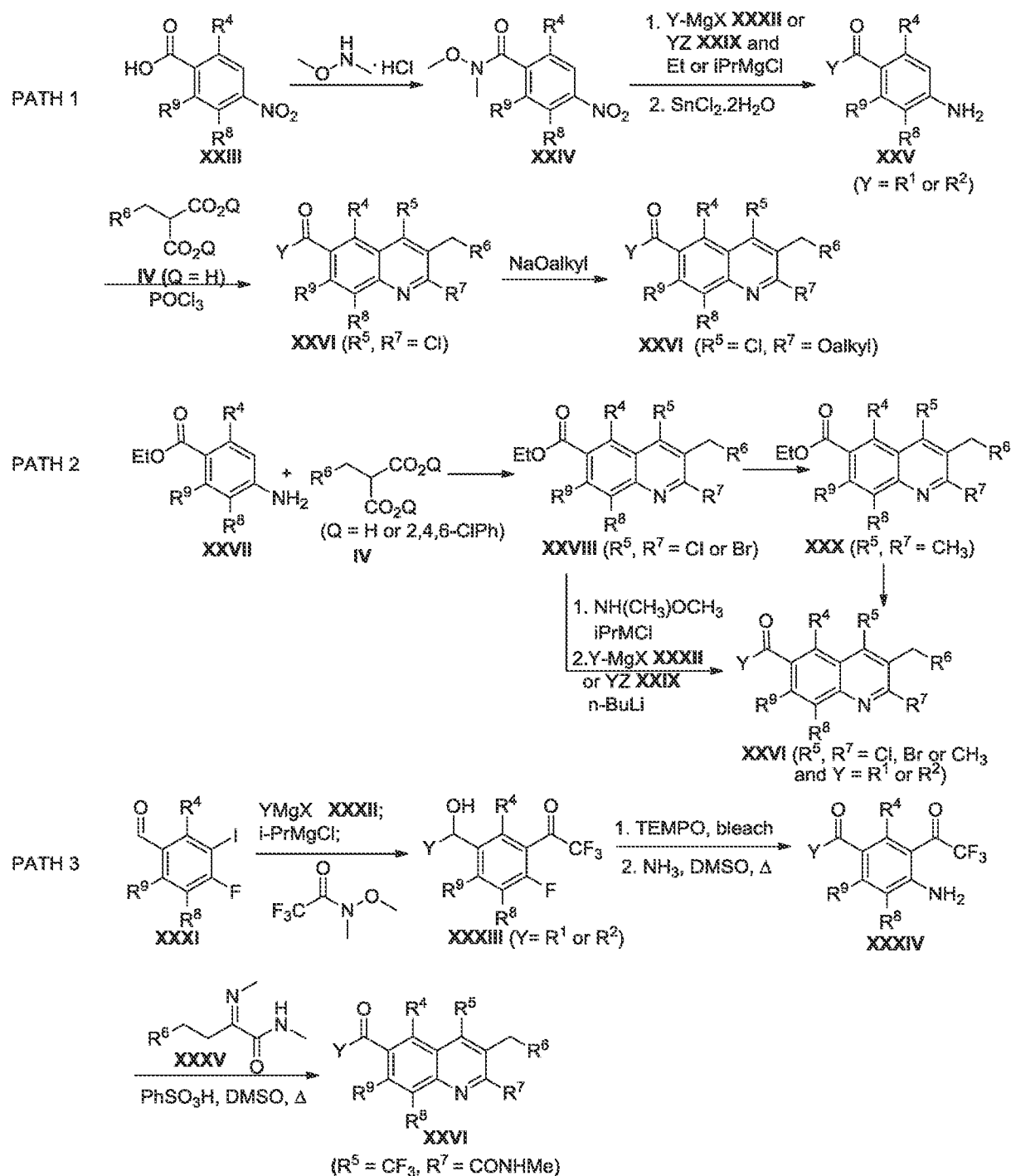
Scheme 3
