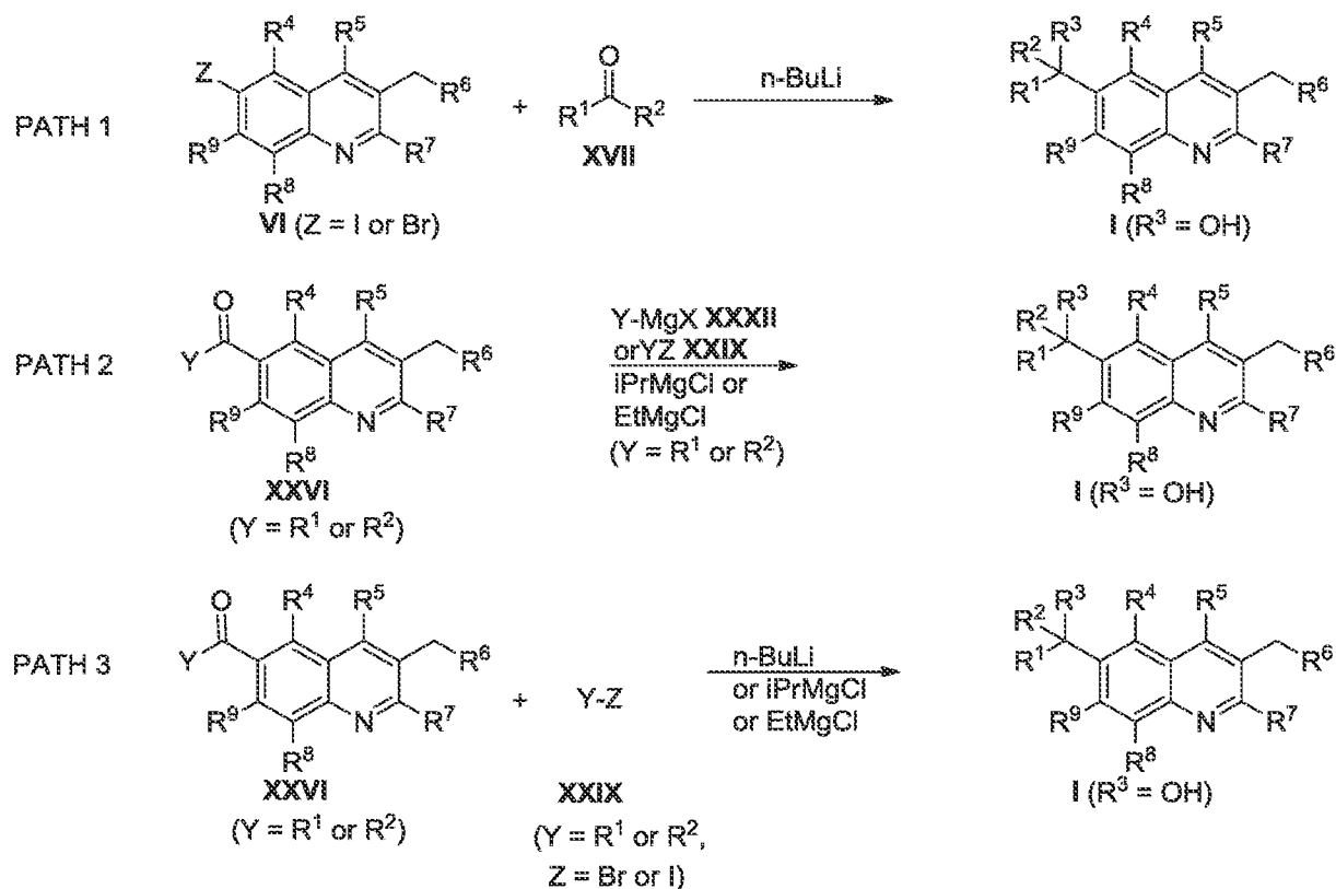
Scheme 5
