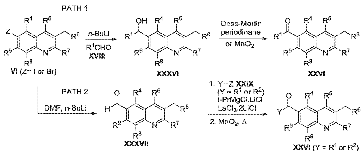
Scheme 4
