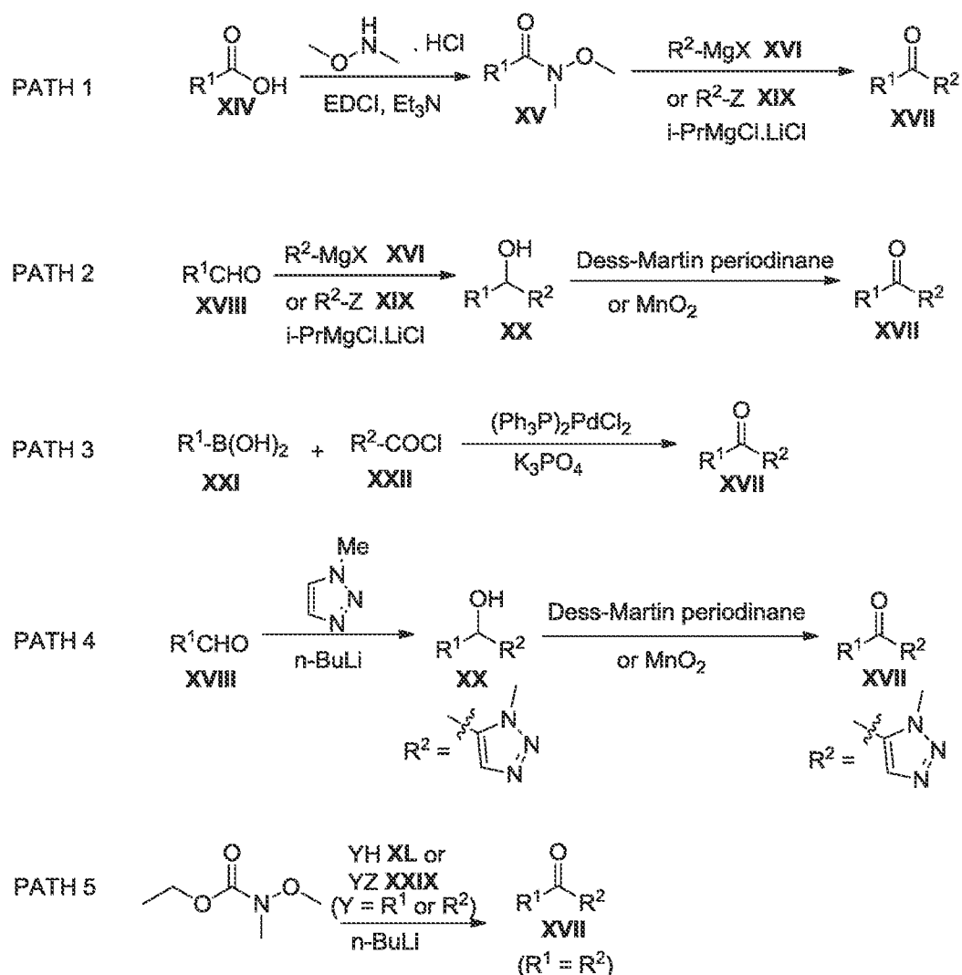
Scheme 2
