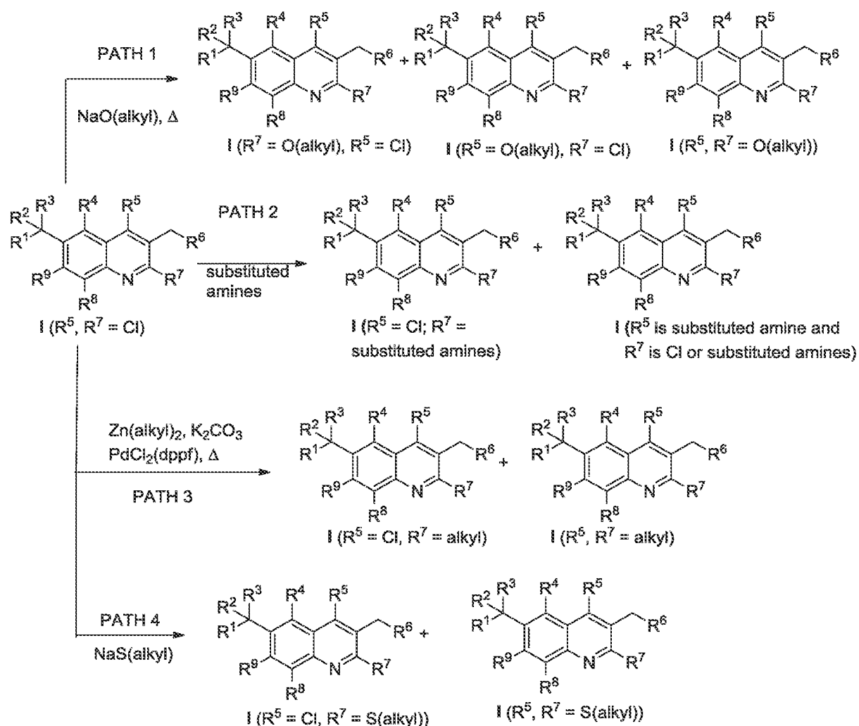
Scheme 6
