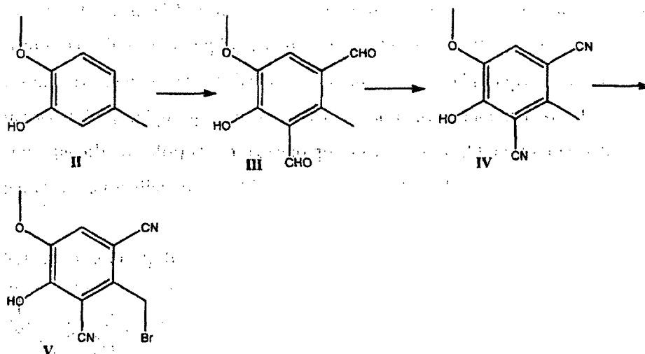
Scheme 1. Starting from 2-methoxy-5-methylphenol
