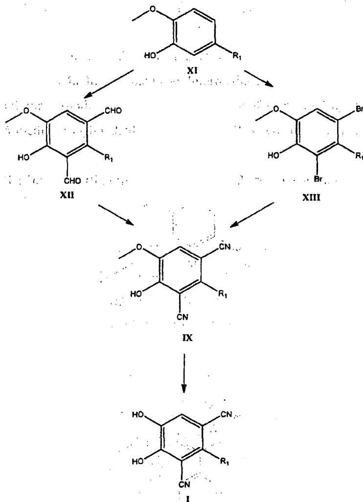
Scheme 3. Starting from a 5-substituted 2-methoxyphenol
