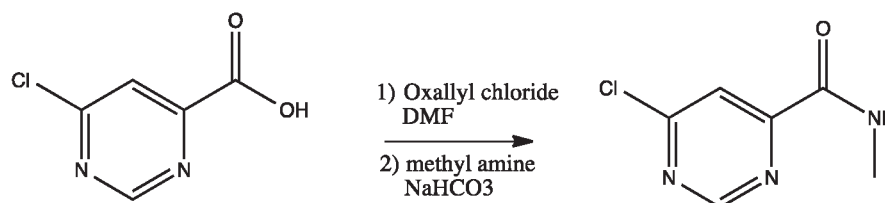
Scheme 13a
