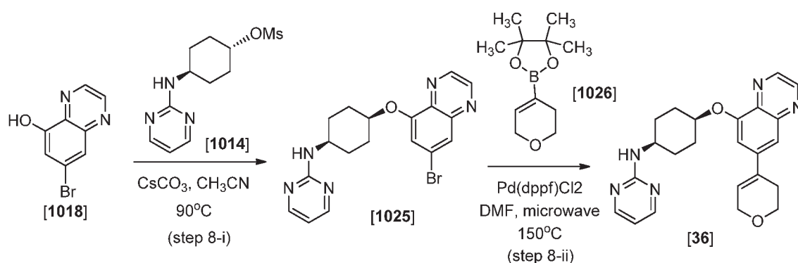
Scheme 8
