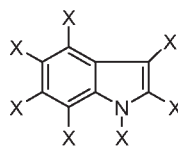
Structure b
