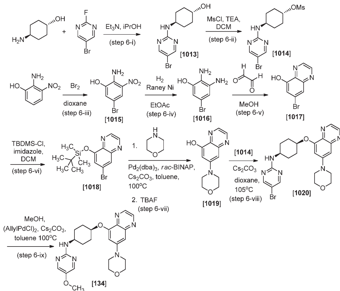
Scheme 6
