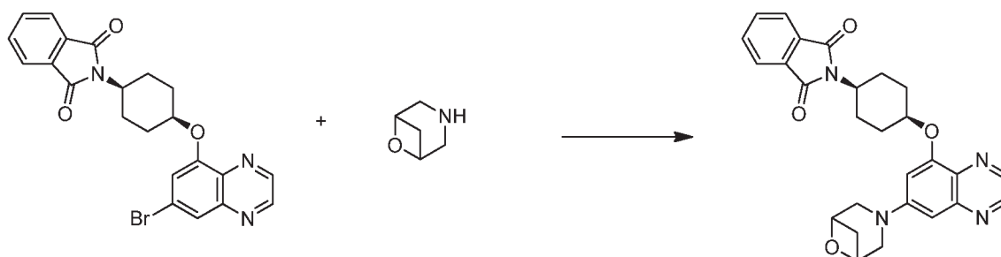
Scheme 10b
