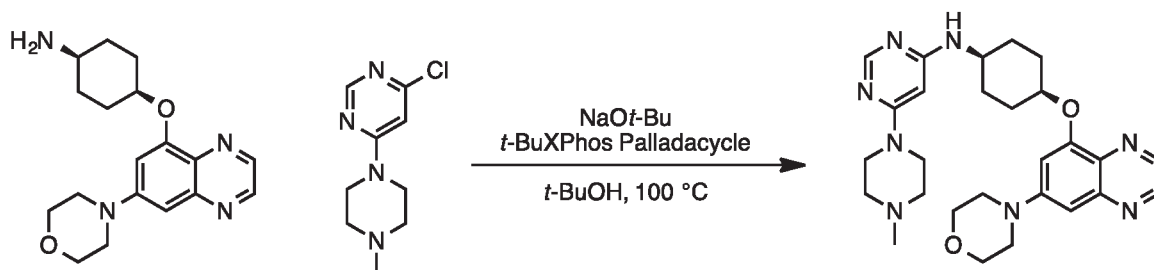
Scheme 11
