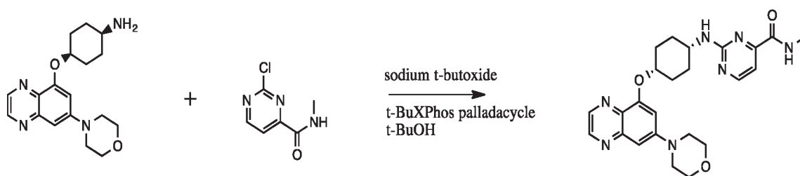
Scheme 14b
