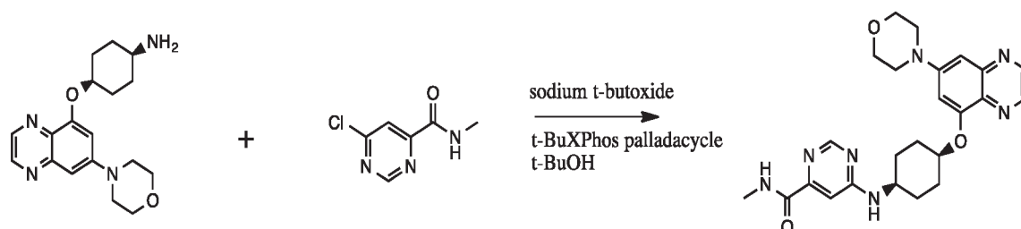
Scheme 13b
