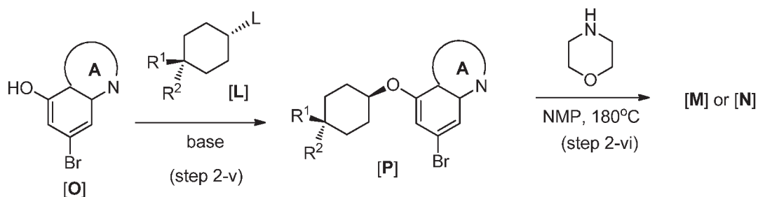
Scheme 2b
