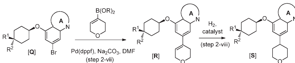
Scheme 2c
