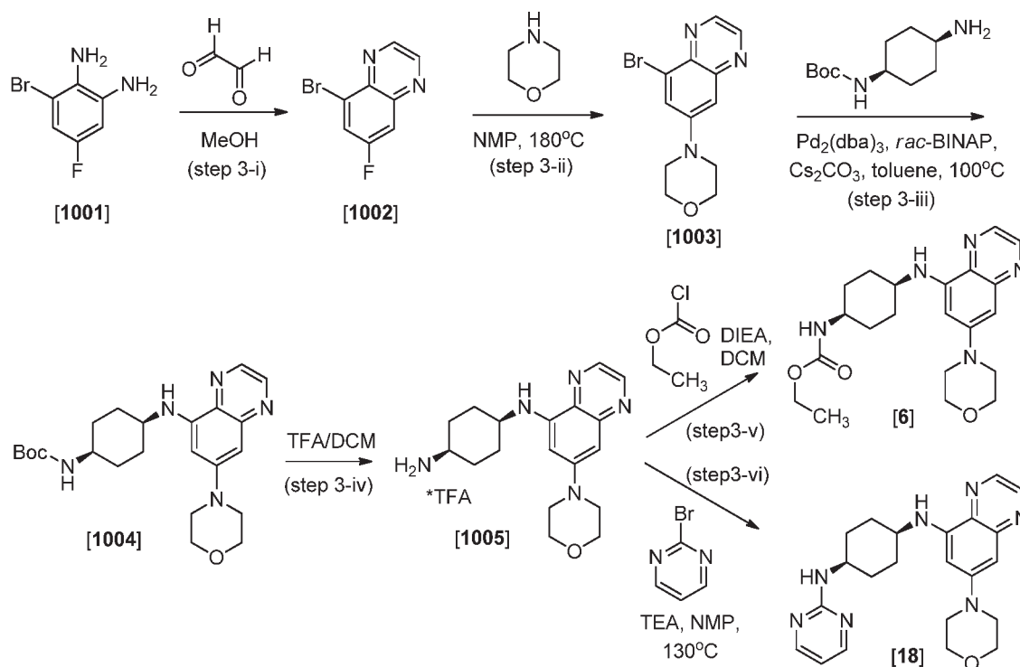
Scheme 3
