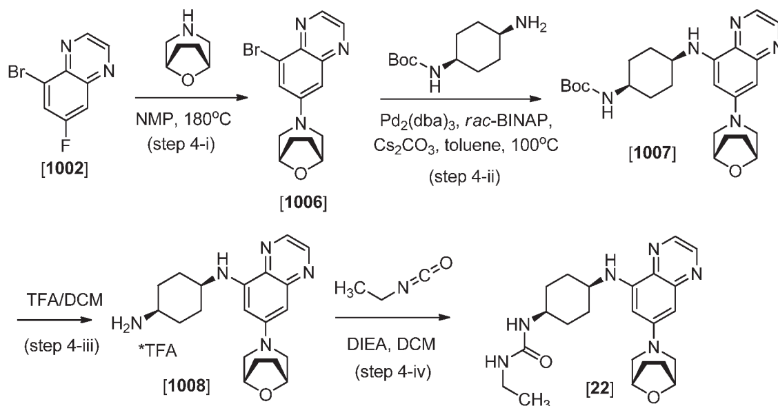
Scheme 4
