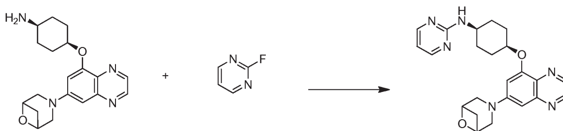
Scheme 10d
