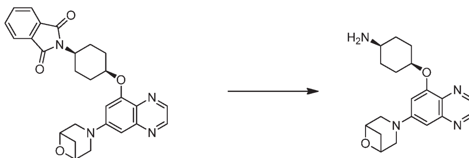
Scheme 10c
