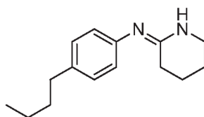
Compound 8
