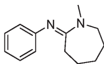
Compound 3
