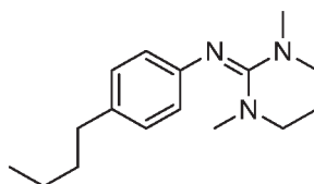
Compound 11
