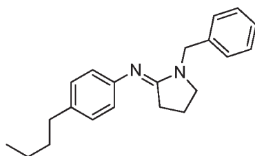
Compound 5
