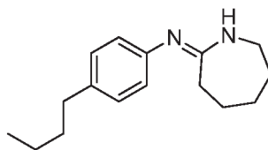
Compound 10
