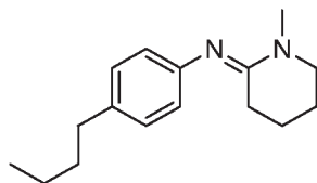
Compound 9
