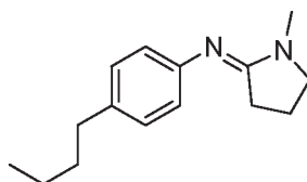
Compound 6
