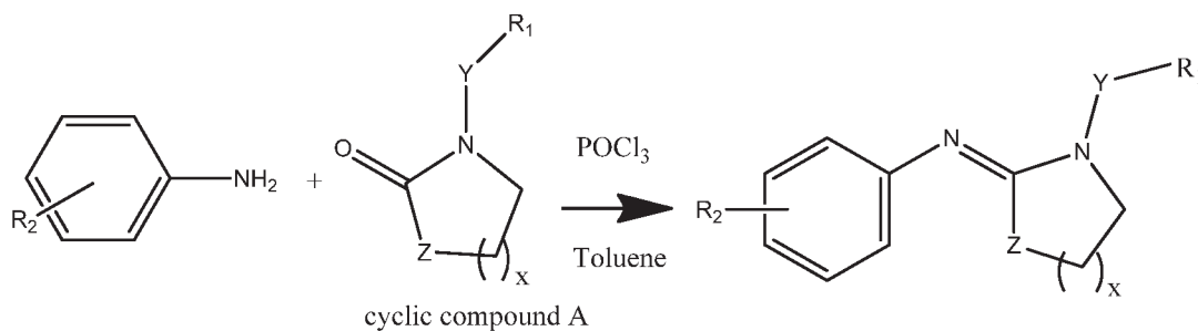
Reaction I
