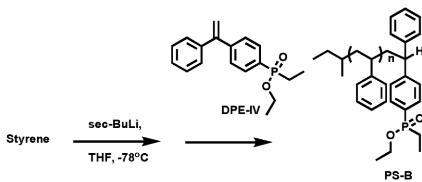
Scheme 10 [0091]
