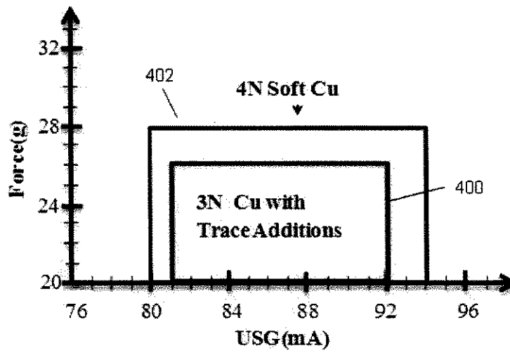
Fig 4(a) - Ball Bond Process Window
