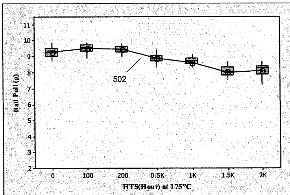
Fig 5(b) - Thermal aged 4N soft Cu 0.8mil wires
