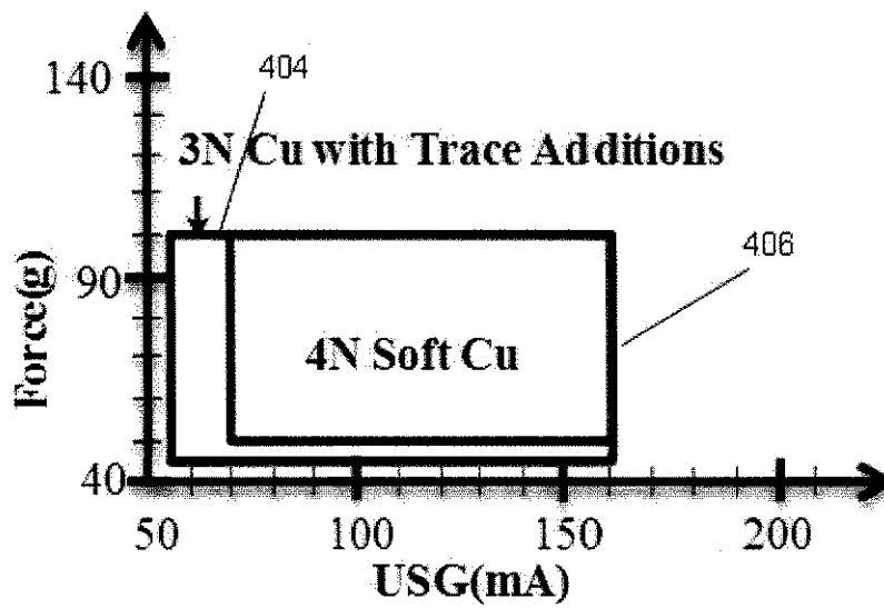
Fig 4(b) - Stitch Bond Process Window
