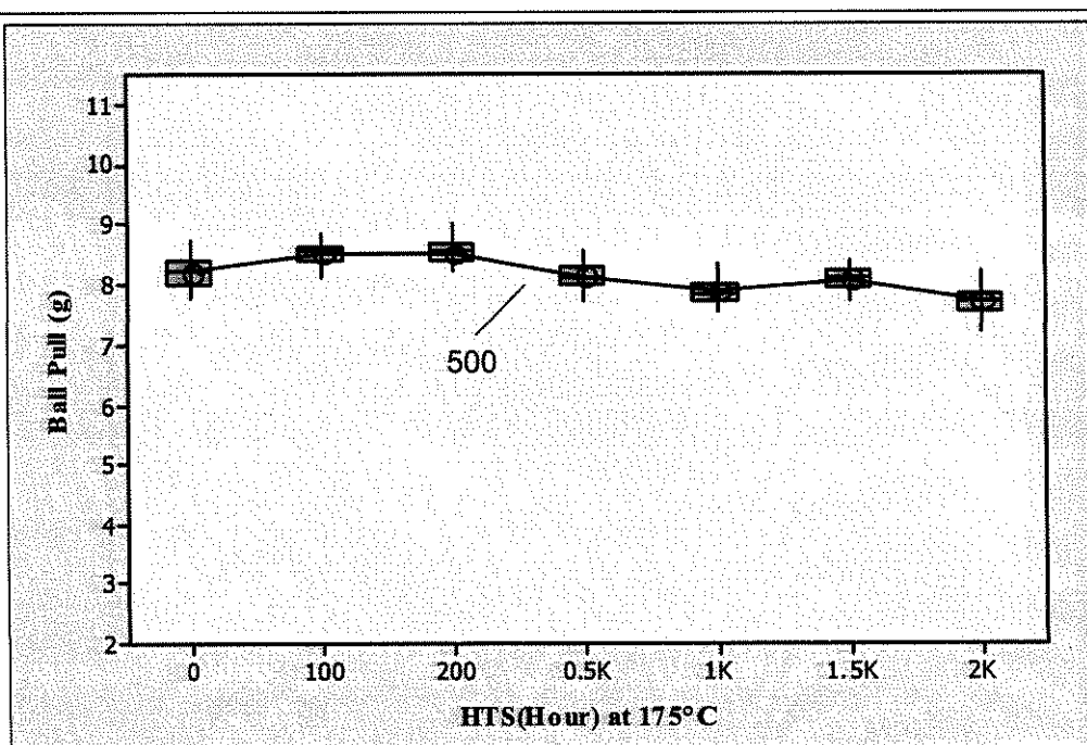
Fig 5(a) – Thermal aged 3N Cu 0.8mil wires with trace additions
