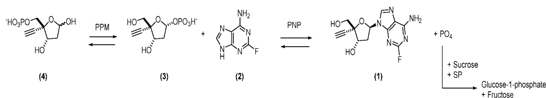
Scheme III. Overall Reaction Scheme to Produce Compound (1)
