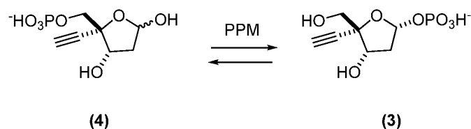
Scheme II. Reaction Catalyzed by Phosphopentomutase (PPM)
