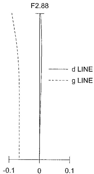
SPHERICAL ABERRATION
