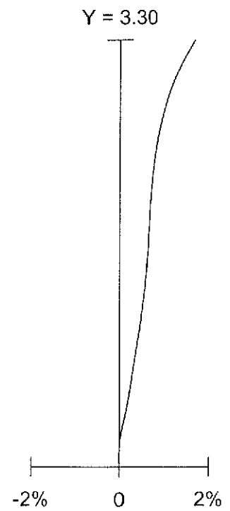
DISTORTION ABERRATION
