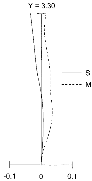
ASTIGMATISM
