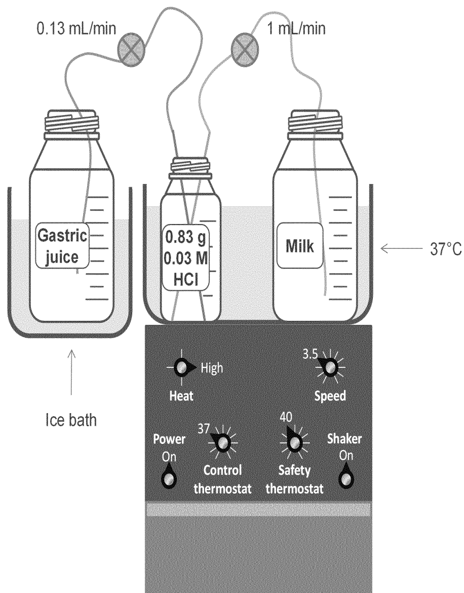
Figure 2 In vitro gastric digestion test set-up
