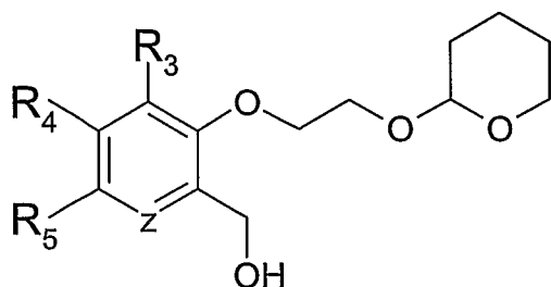
Formula (XIX)
