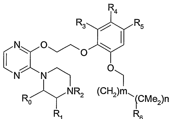
Formula (Ia)
