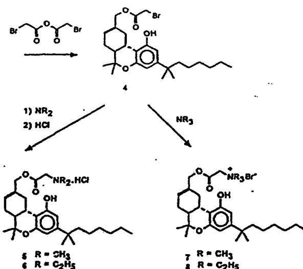
Scheme II
