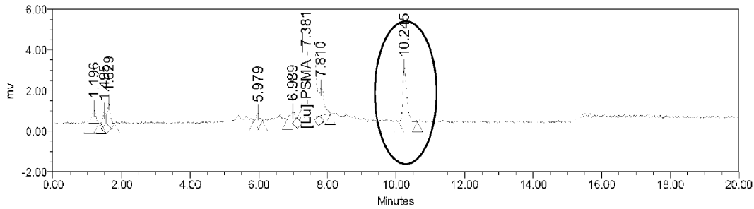
FIG. 1C Auto-Scaled Chromatogram
