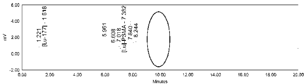
FIG. 1C Auto-Scaled Chromatogram
