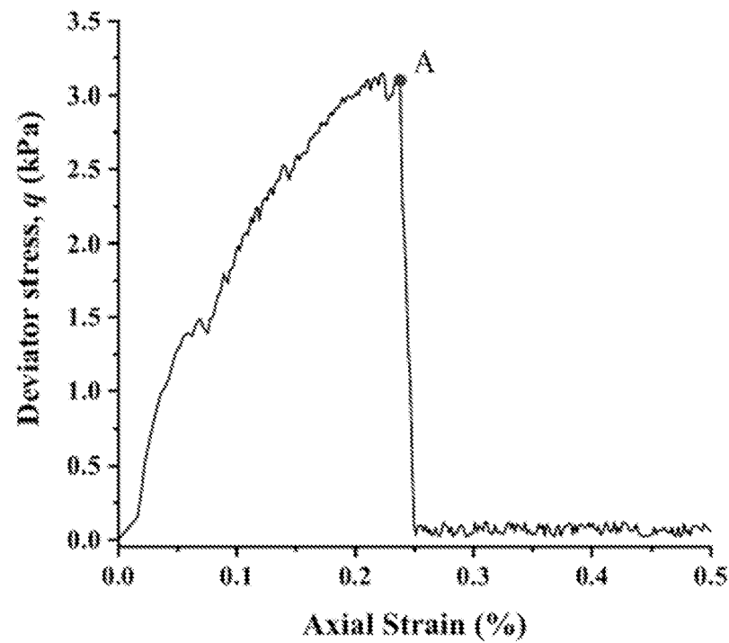
(a) Stress-strain response
