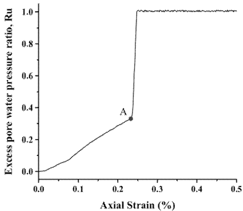
(b) Pore water pressure response
