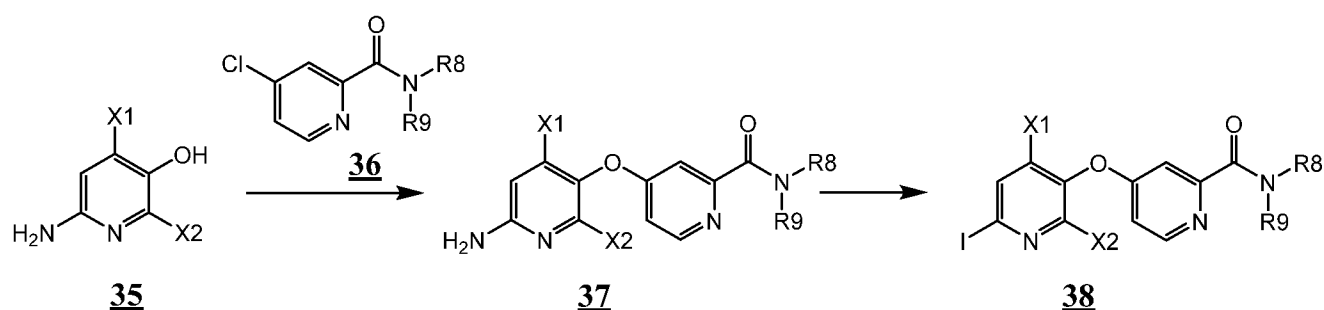
Scheme 6
