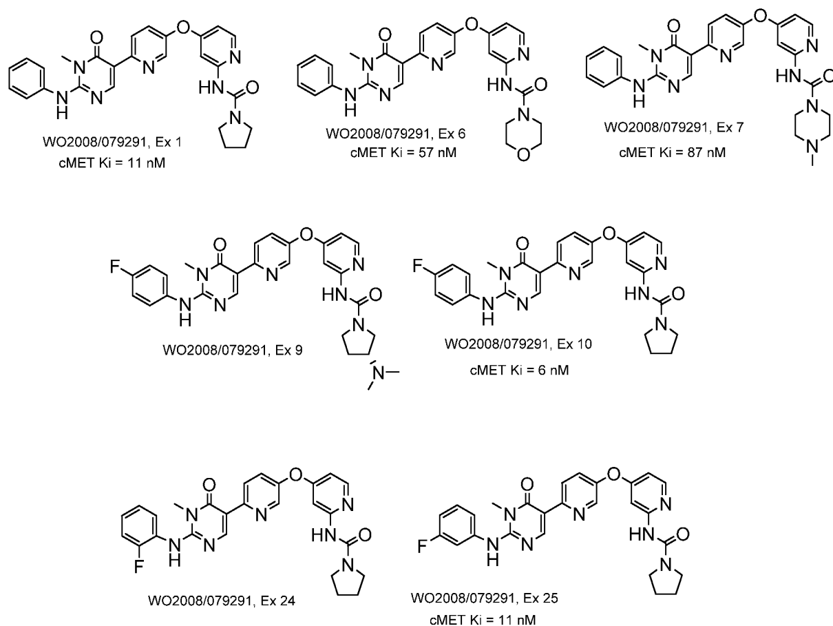
Figure 1. cMET inhibitors of WO2008/079291.
