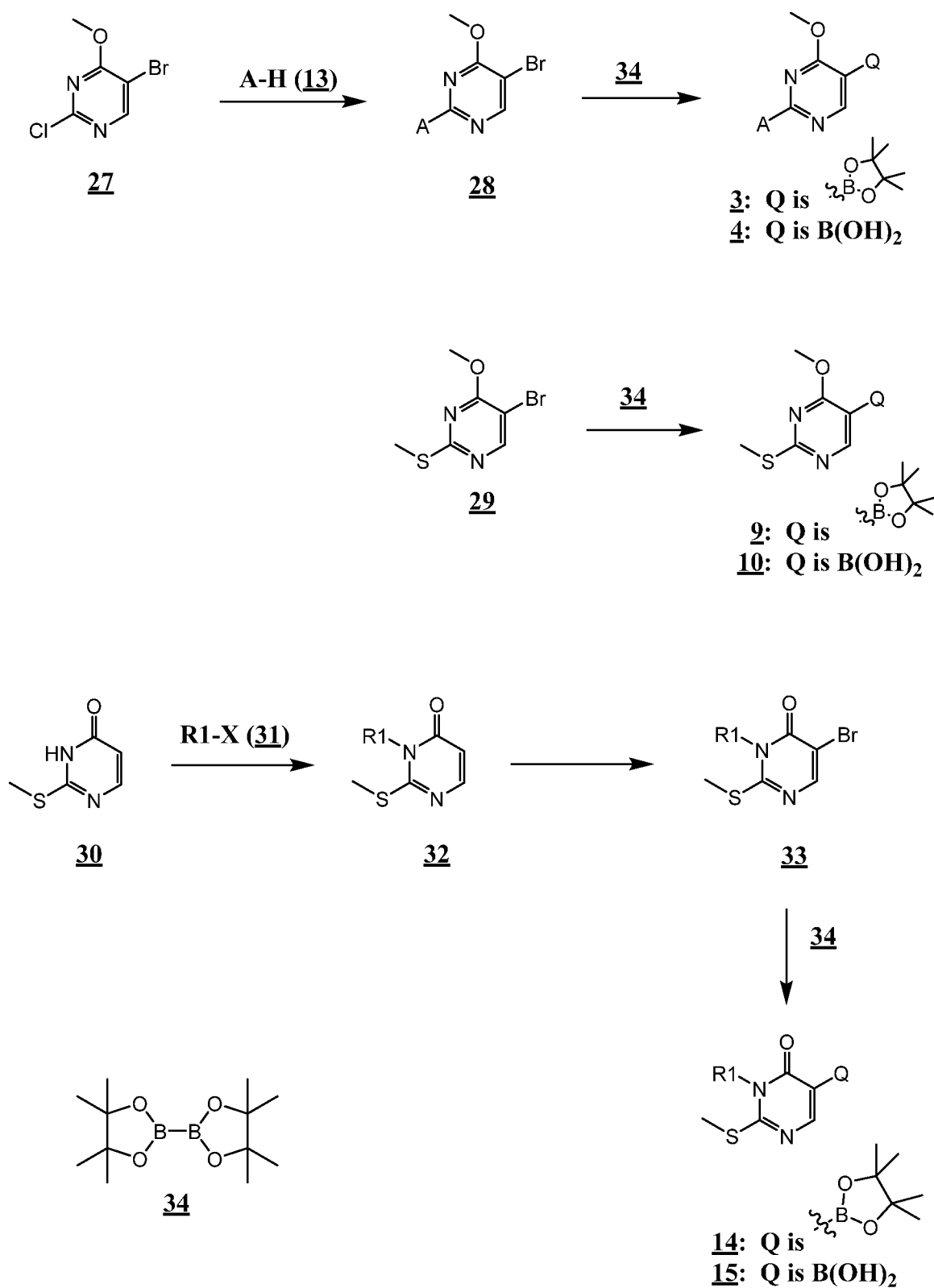
Scheme 5
