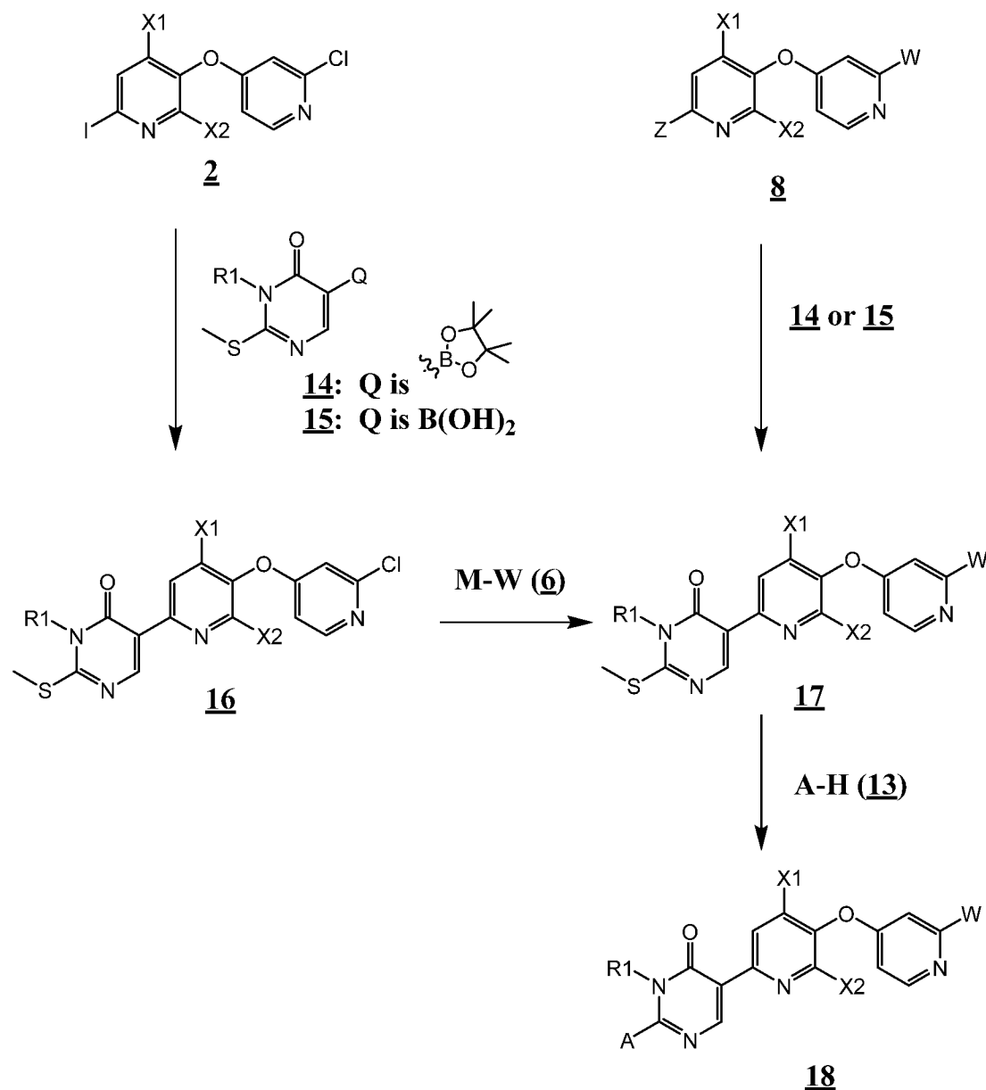
Scheme 2
