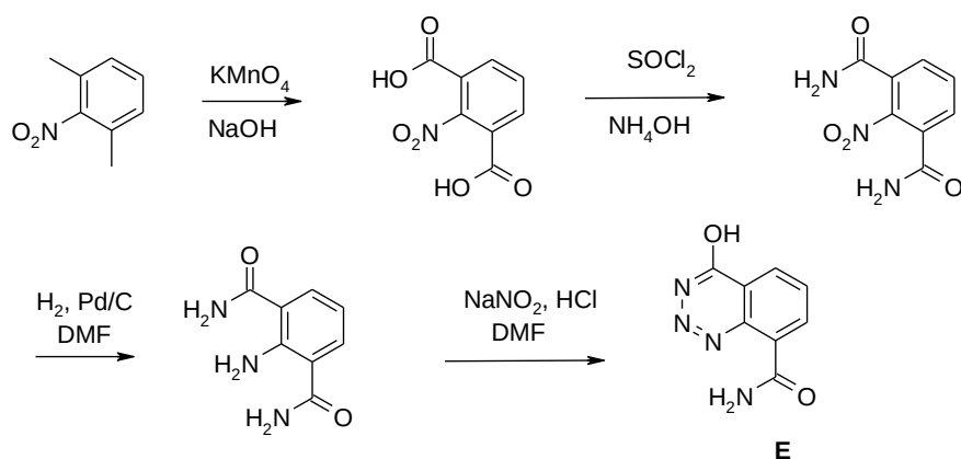
Scheme 3: 2-Nitro- m -xylene was treated with potassium permanganate in the presence of NaOH in water to afford 2-nitroisophthalic acid intermediate. The diacid was refluxed with thionyl chloride in DMF, followed by addition of aqueous ammonia in THF to give 2-nitro isophthalamide, which was then hydrogenated using Pd/C to give the 2-amino isophthalamide intermediate. Cyclization of 2-amino isophthalamide proceeded in DMF using sodium nitrite in 0.5M Hydrochloric acid gave the desired 4-Oxo-3,4-dihydro-benzo[d][1,2,3]triazine-8-carboxamide E .
