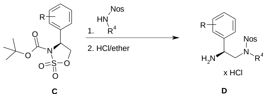
Scheme 2: Nucleophilic attack of intermediate C (WO12/69146) with a nosyl-protected primary amine followed by Boc-deprotection with hydrochloric acid afforded the desired amine hydrochloride salt intermediate D .
