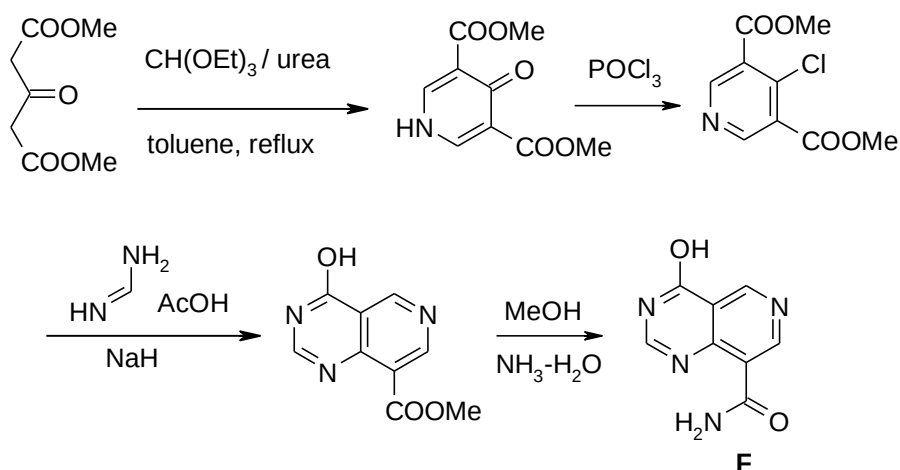
Scheme 4: A mixture of dimethyl 3-oxopentanedioate, triethoxymethane and urea in toluene was refluxed to afford dimethyl 4-oxo-1,4-dihydropyridine-3,5-dicarboxylate as a precipitate. This intermediate was then refluxed in phosphoryl chloride to give the 4-chloropyridine intermediate. The solution of diester and formimidamide acetate in 1,4-dioxane were treated with sodium hydride to afford 4-hydroxypyrido[4,3-d]pyrimidine-8-carboxamide F .
