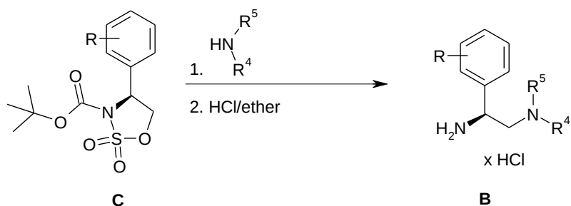
Scheme 1B: Nucleophilic attack of intermediate C (WO12/69146) with a secondary alkyl amine followed by Boc-deprotection with hydrochloric acid afforded the desired amine hydrochloride salt intermediate B .
