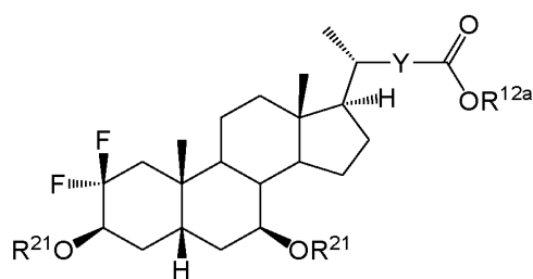
(XXI)
