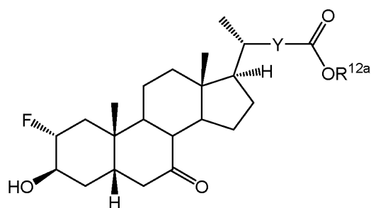
(XIIa)
