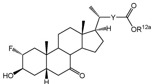
(XIIa)
