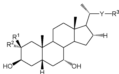
(IC)
