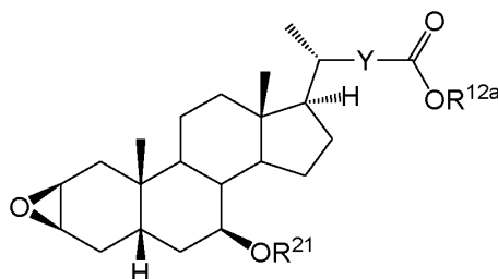
(XXVIa)
