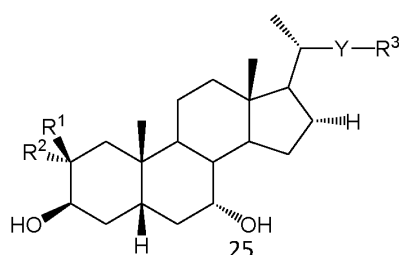
(IC)
