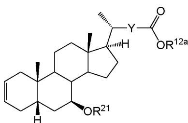
(XXVI)
