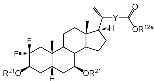
(XXI)
