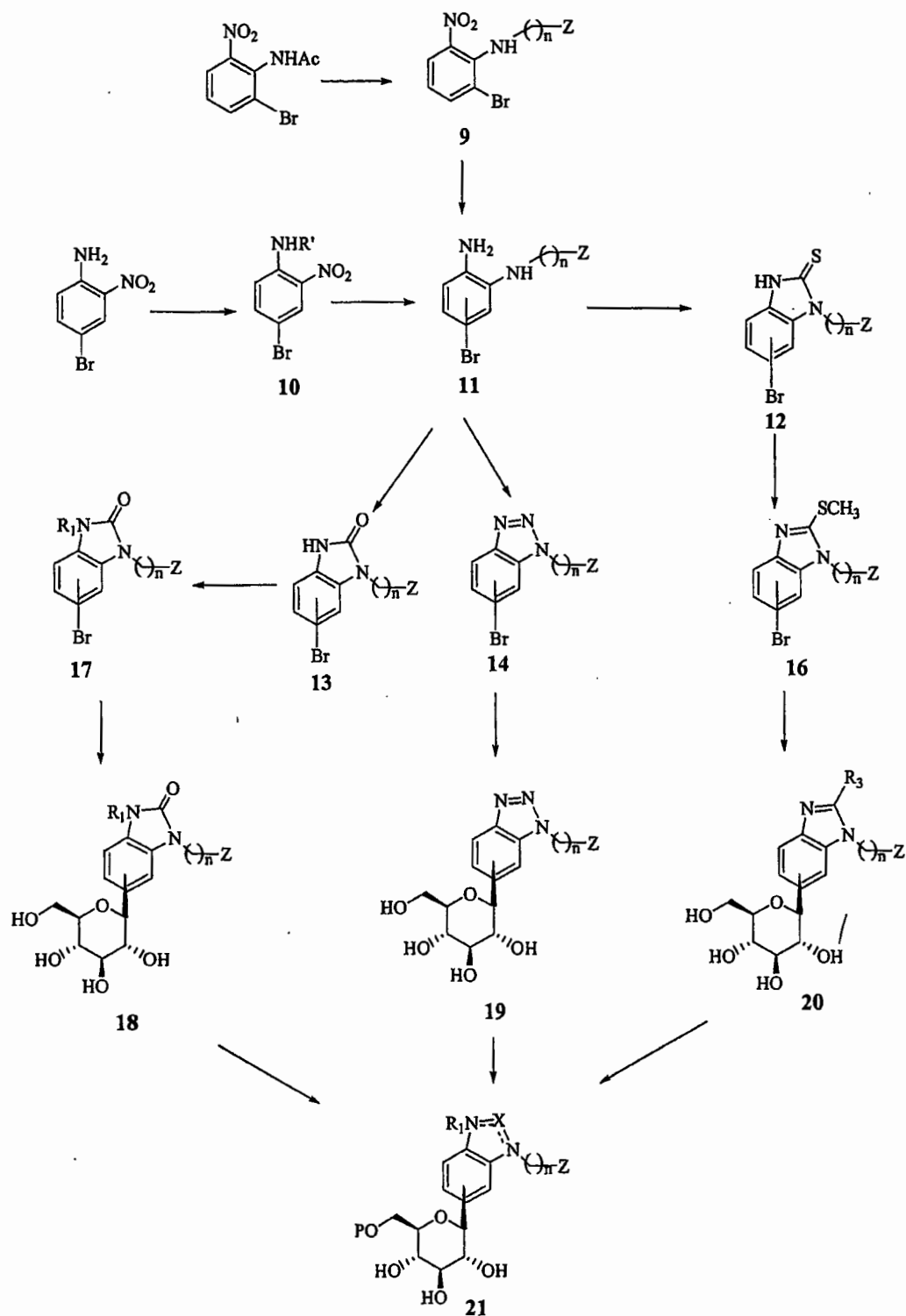
Scheme 2
