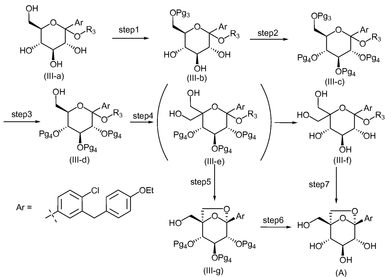
Scheme 3
