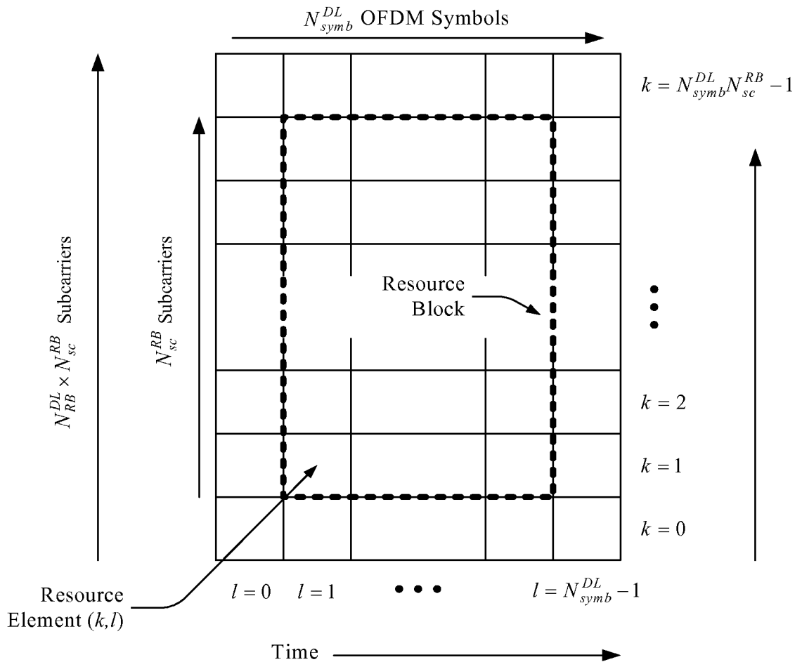
Diagram 1: Downlink Resource Grid
