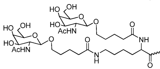
Formula XVI,
