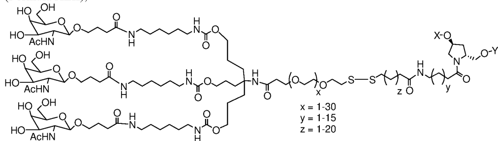
(Formula XLII),
