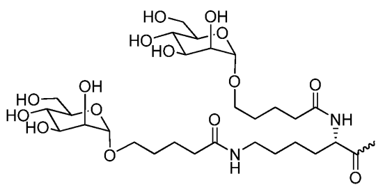
Formula XXI,
