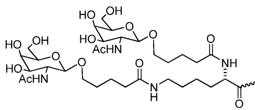
Formula XIV,
