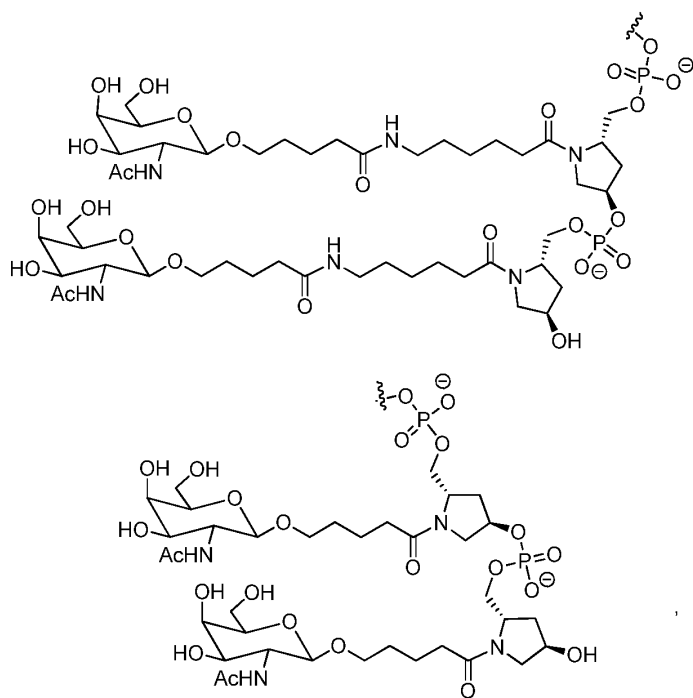
Formula XXXI;
