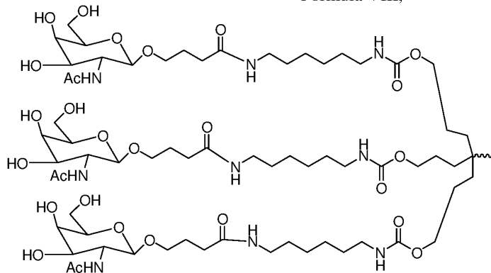
Formula VIII,
