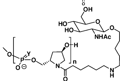
Formula XXIII;
