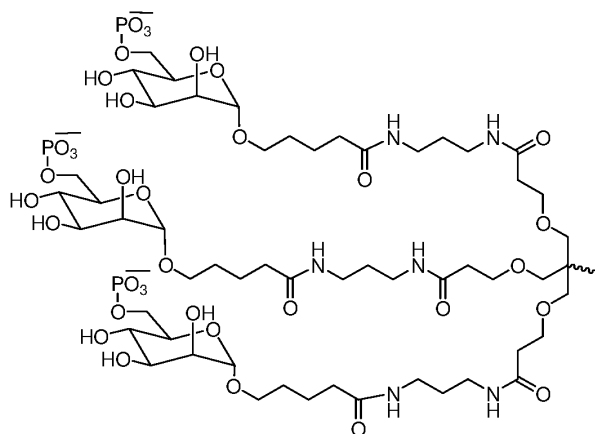
Formula XI,
