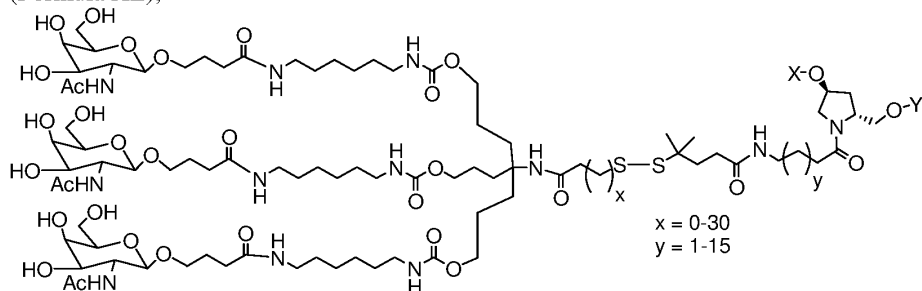
(Formula XL),
