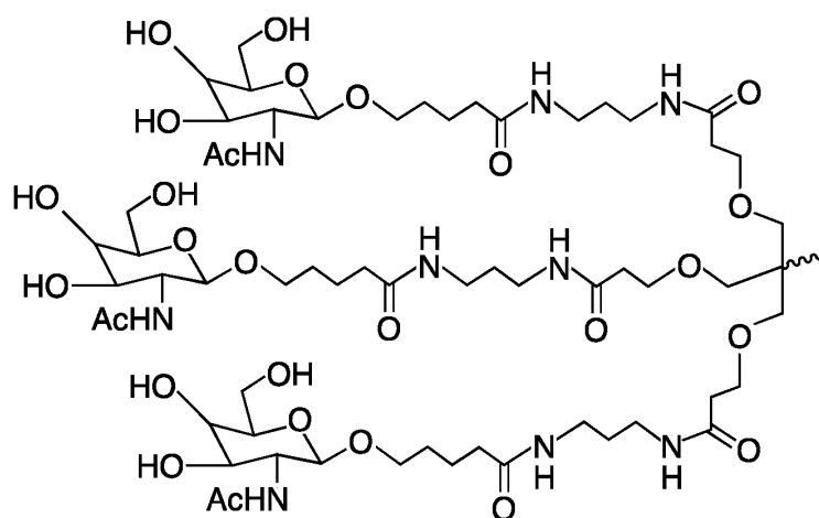
Formula II.
