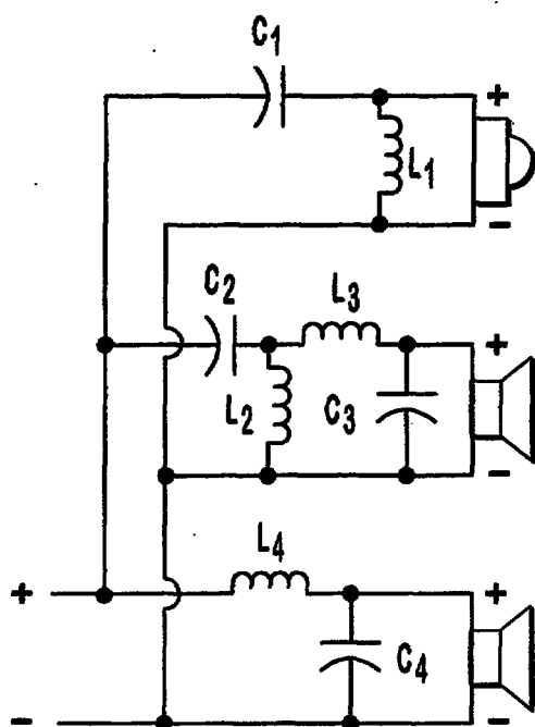
FIG. 2 (PRIOR ART)
