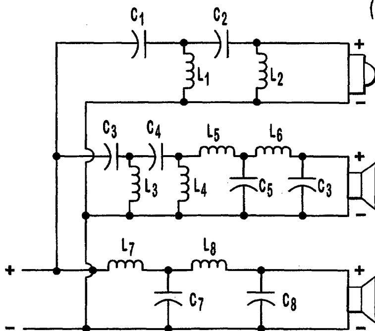
FIG. 4 (PRIOR ART)
