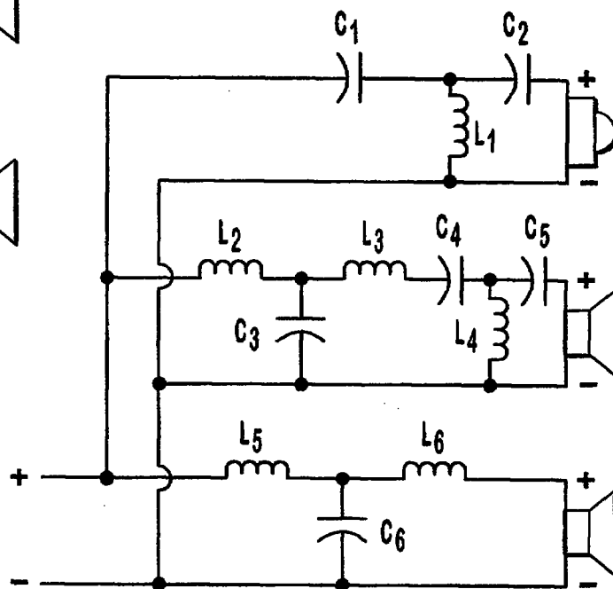
FIG. 3 (PRIOR ART)
