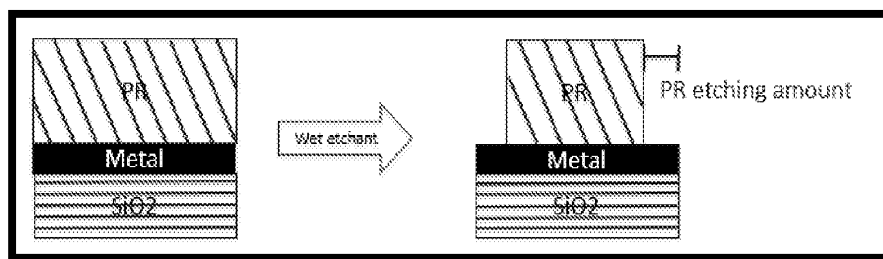
FIG. 1. Photoresist Removal
