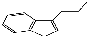
3-propyl-1H-indene
