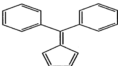
6,6-diphenylpentafulvene
