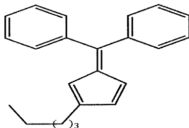
2-(pentyl)-6,6-diphenylpentafulvene
