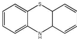
Phenothiazine (PTZ)
