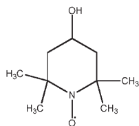
4-hydroxy Tempo
